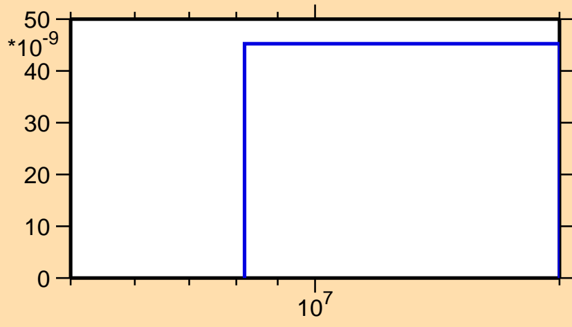
\sigma vs. E for ^{118}\text{Te}(n,p\alpha)
