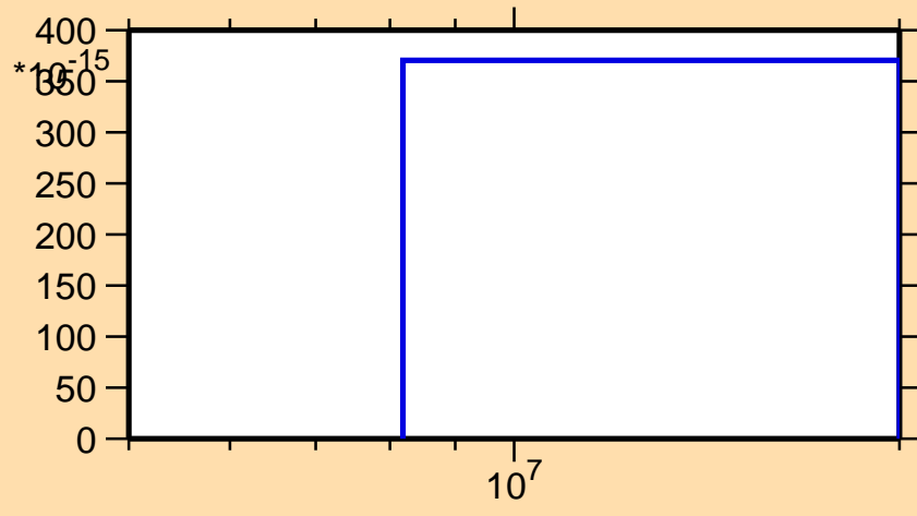
\sigma vs. E for ^{118}\text{Te}(\text{mt } 45)
