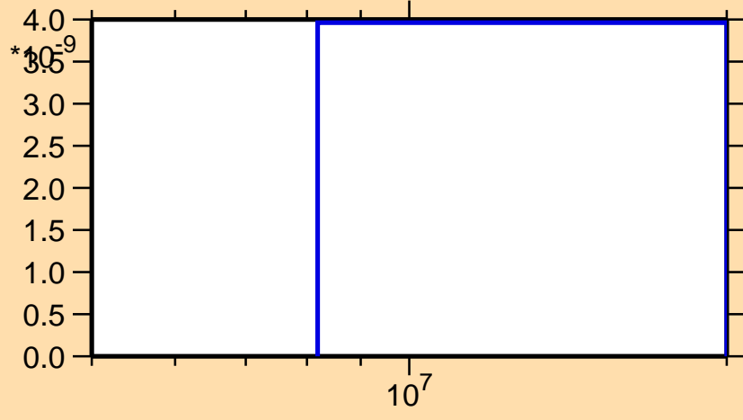
\sigma vs. E for ^{118}\text{Te}(n,2np)
