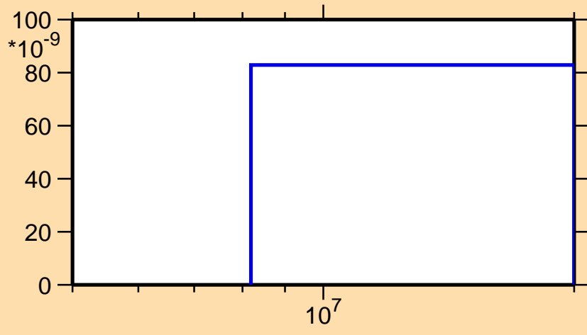
\sigma vs. E for ^{118}\text{Te}(n,\text{He3})
