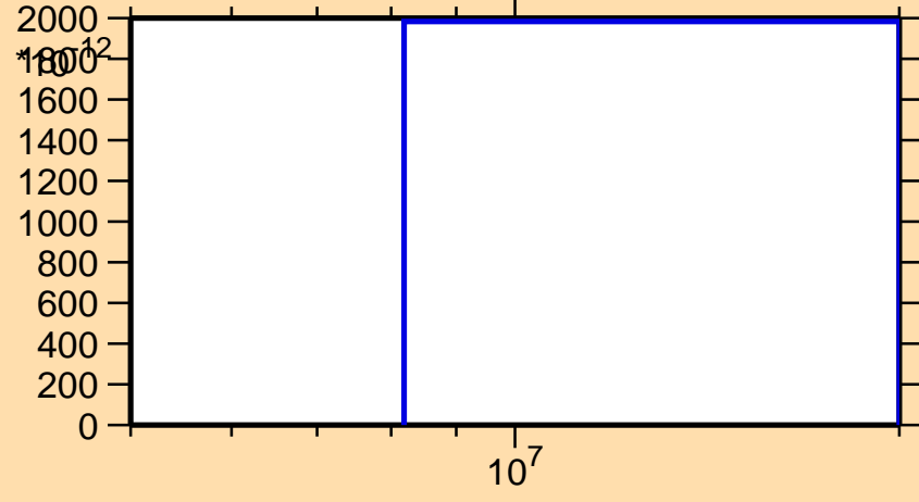
\sigma vs. E for ^{118}\text{Te}(n,\text{nd})
