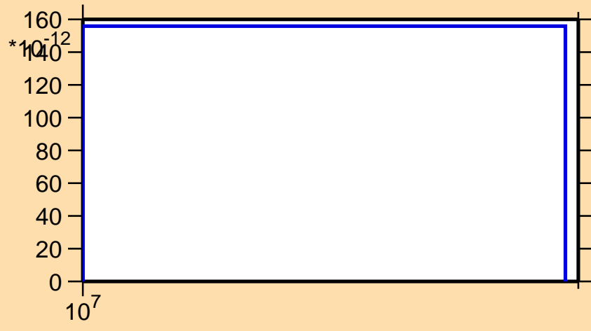
\sigma vs. E for ^{119}\text{Te}(n,pd)
