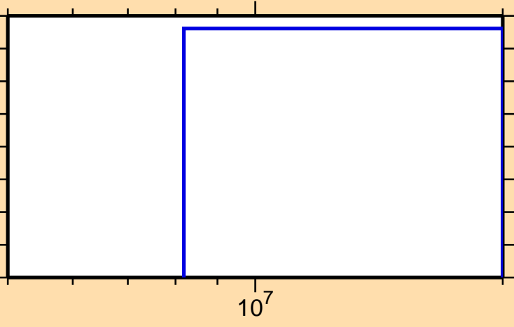
\sigma vs. E for ^{119}\text{Te} (mt 45)
