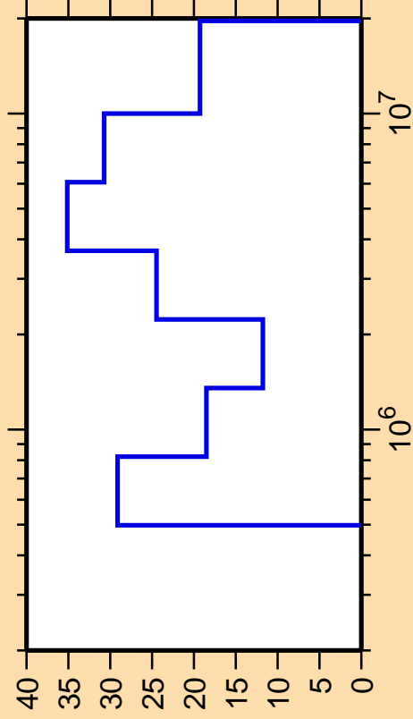
\Delta\sigma/\sigma vs. E for ^{120}\text{Te}(n,n_1)
