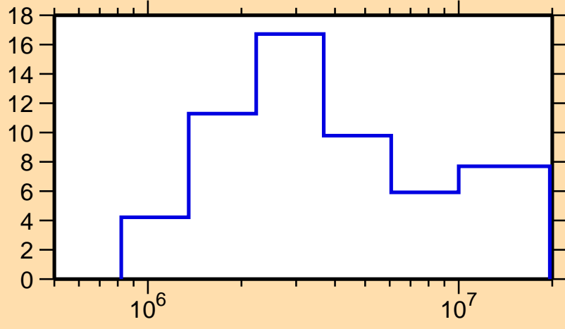
\Delta\sigma/\sigma vs. E for ^{120}\text{Te}(n,el.)
