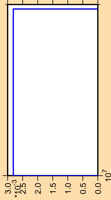
\Delta\sigma/\sigma vs. E for ^{120}\text{Te}(\text{mt117})
