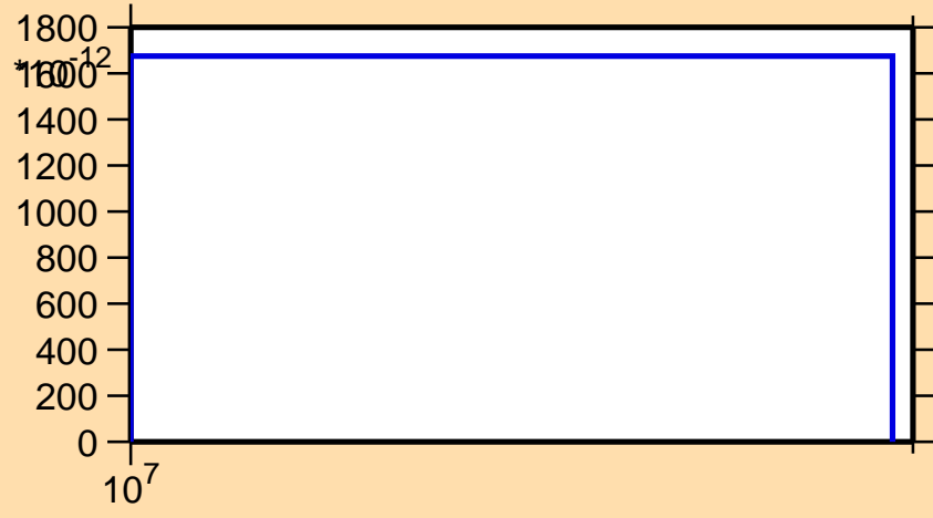
\sigma vs. E for ^{120}\text{Te}(n,\text{nd})
