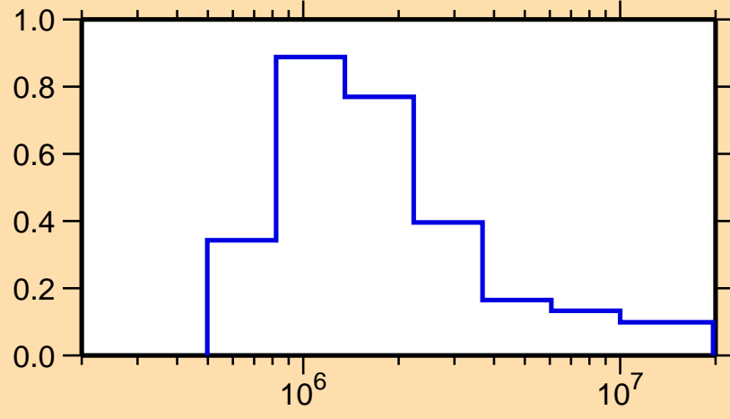
\sigma vs. E for ^{120}\text{Te}(n,n_1)
