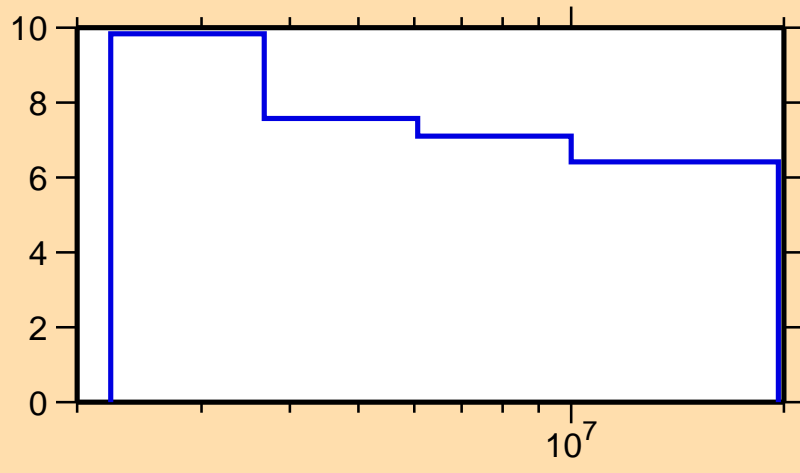
\Delta\sigma/\sigma vs. E for ^{120}\text{Te}(n,n\text{onel.})
