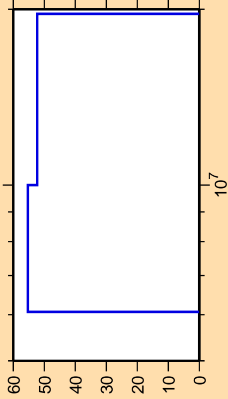
\Delta\sigma/\sigma vs. E for ^{120}\text{Te}(n,np)
