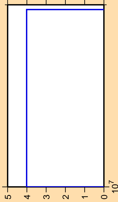
\Delta\sigma/\sigma vs. E for ^{120}\text{Te}(n,nt)
