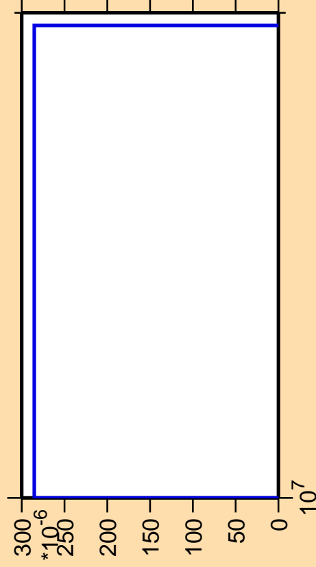
\Delta\sigma/\sigma vs. E for ^{120}\text{Te} (mt 45)
