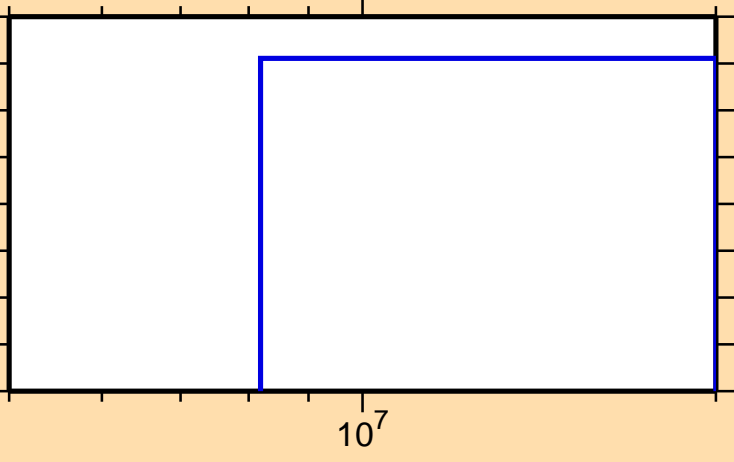
\sigma vs. E for ^{120}\text{Te}(n,\text{pt})
