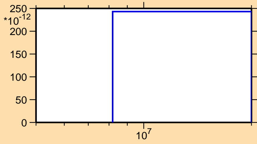
\sigma vs. E for ^{120}\text{Te}(n,pd)
