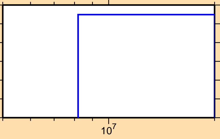
\sigma vs. E for ^{120}\text{Te}(n,\text{He}3)
