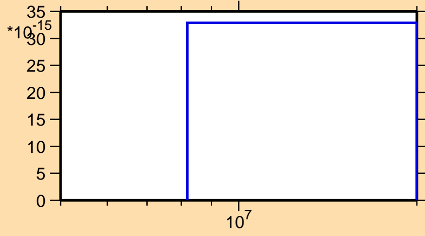
\sigma vs. E for ^{121}\text{Te} (mt 34)
