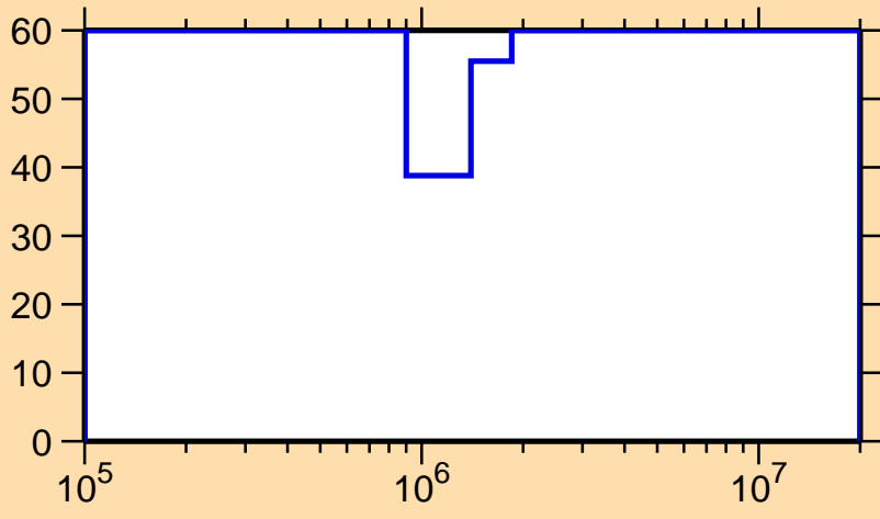
\Delta\sigma/\sigma vs. E for ^{121}\text{Te}(n,n_1)
