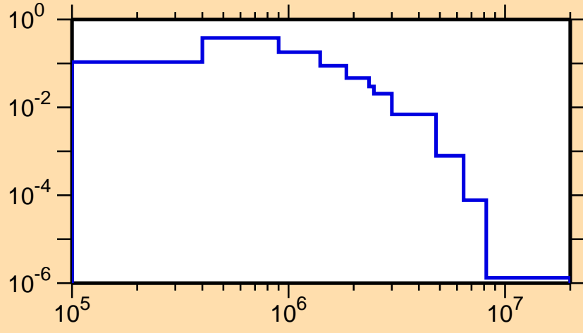
\sigma vs. E for ^{121}\text{Te}(n,n_1)
