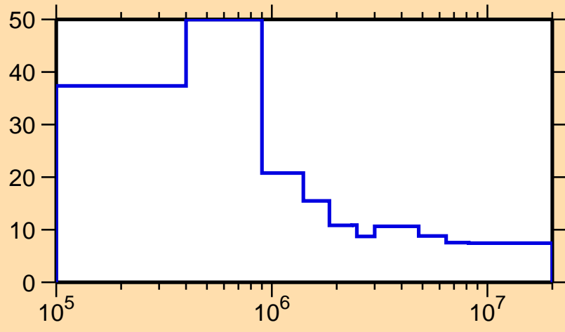
\Delta\sigma/\sigma vs. E for ^{121}\text{Te}(n,\text{nonel.})
