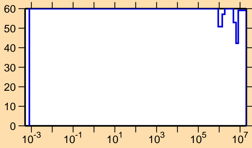
\Delta\sigma/\sigma vs. E for ^{121}\text{Te}(n,p)
