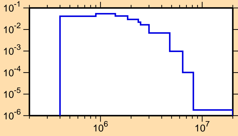
\sigma vs. E for ^{121}\text{Te}(n,n_4)
