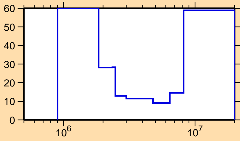
\Delta\sigma/\sigma vs. E for ^{121}\text{Te}(n,n\text{cont.})
