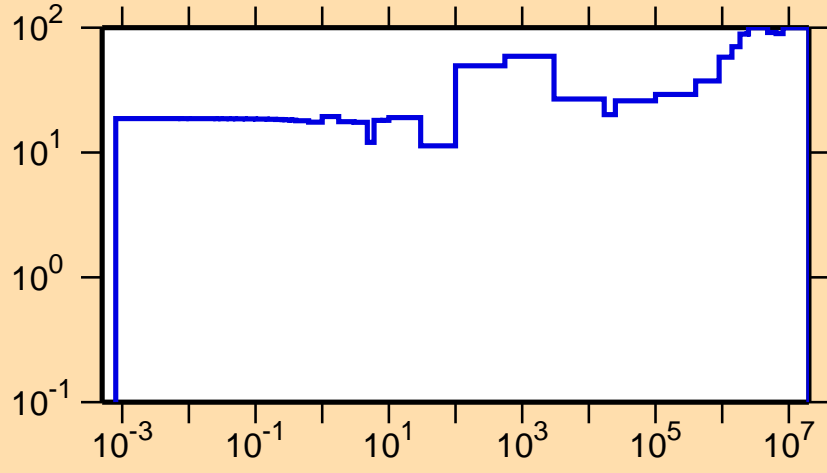
\Delta\sigma/\sigma vs. E for ^{121}\text{Te}(n,\gamma)
