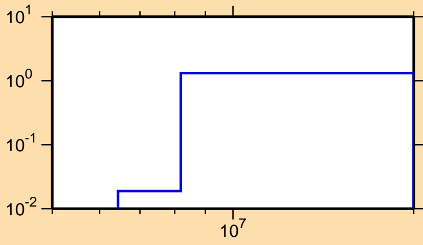
\sigma vs. E for ^{121}\text{Te}(n,2n)
