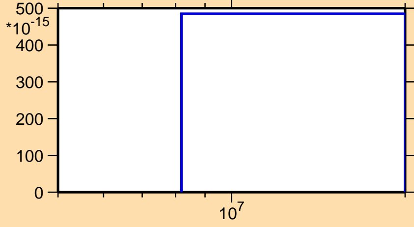
\sigma vs. E for ^{121}\text{Te}(n,pd)
