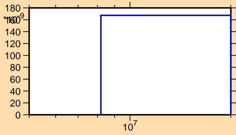
\sigma vs. E for ^{121}\text{Te}(n,2np)
