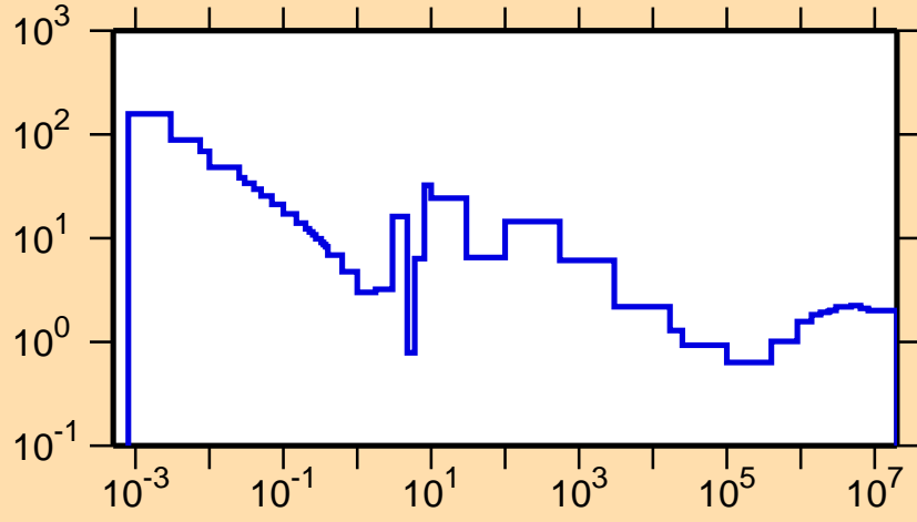
\sigma vs. E for ^{121}\text{Te}(n,\text{nonel.})
