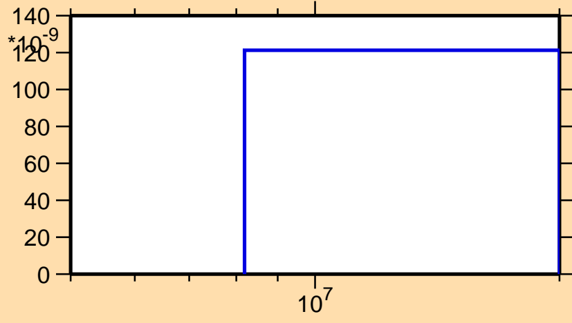
\sigma vs. E for ^{121}\text{Te}(n,\text{nd})
