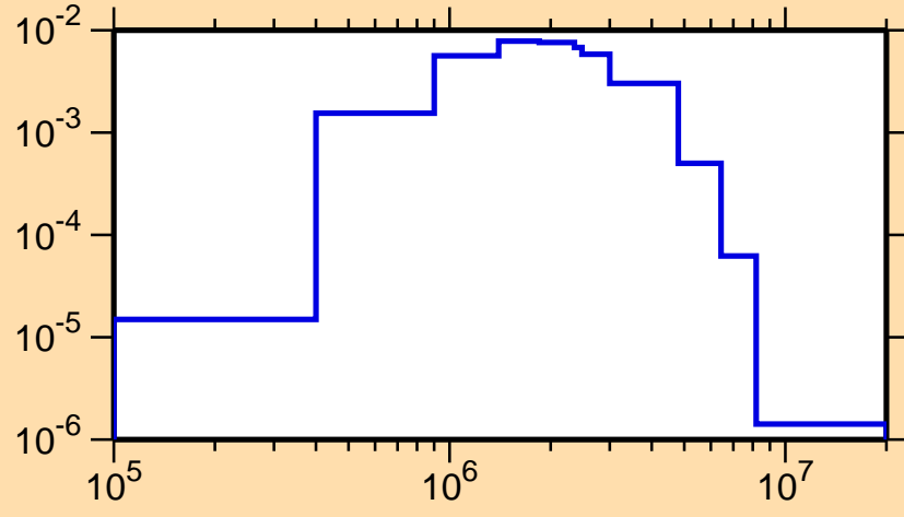
\sigma vs. E for ^{121}\text{Te}(n,n_2)
