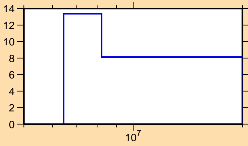
\Delta\sigma/\sigma vs. E for ^{121}\text{Te}(n,\text{el.})
