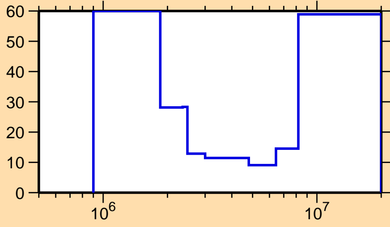
\Delta\sigma/\sigma vs. E for ^{121}\text{Te}(n,n\text{cont.})
