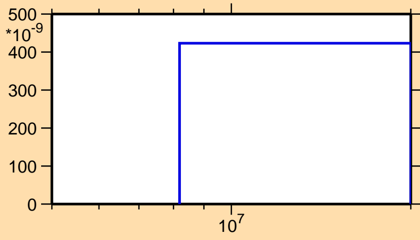
\sigma vs. E for ^{121}\text{Te}(n,2n\alpha)
