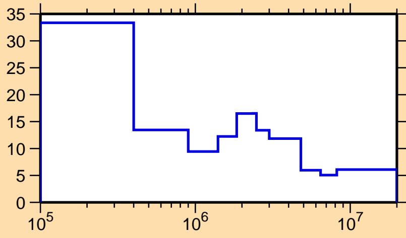
\Delta\sigma/\sigma vs. E for ^{121}\text{Te}(n,\text{tot.})
