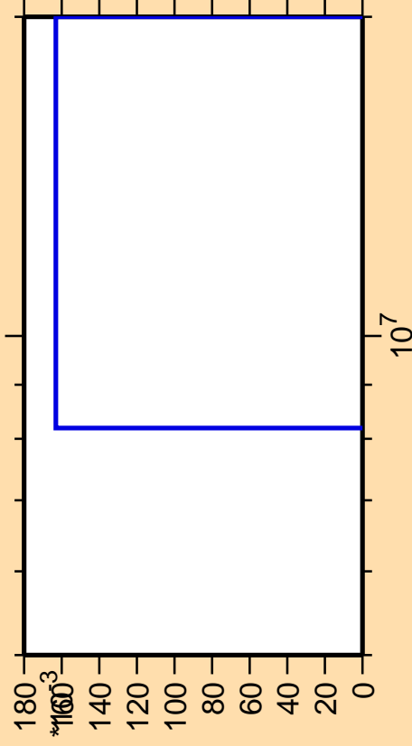
\Delta\sigma/\sigma vs. E for ^{121}\text{Te} (mt 34)
