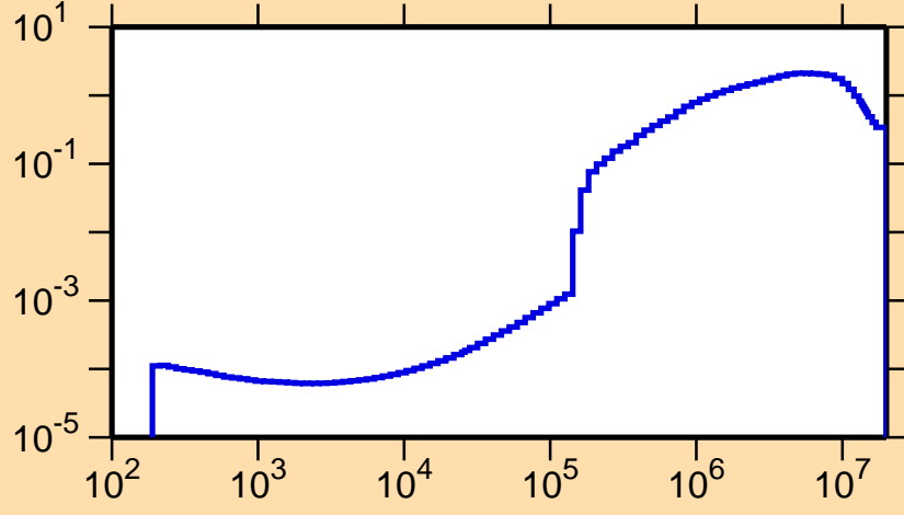
\sigma vs. E for ^{121}\text{Te}(n,\text{inel.})
