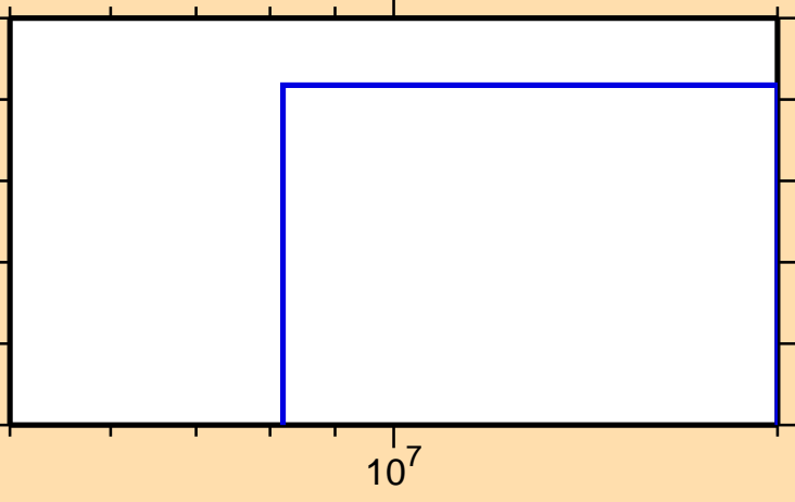
\sigma vs. E for ^{121}\text{Te}(n,\text{nd})
