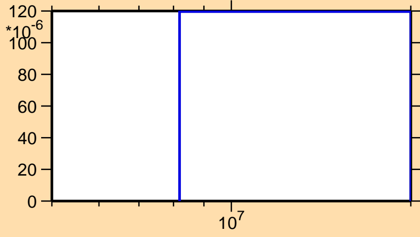
\sigma vs. E for ^{121}\text{Te}(n,t)
