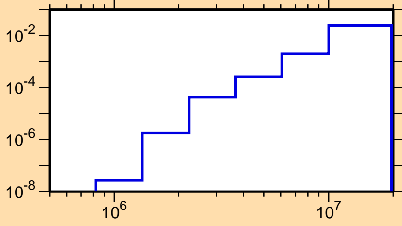
\sigma vs. E for ^{123}\text{Te}(n,p)
