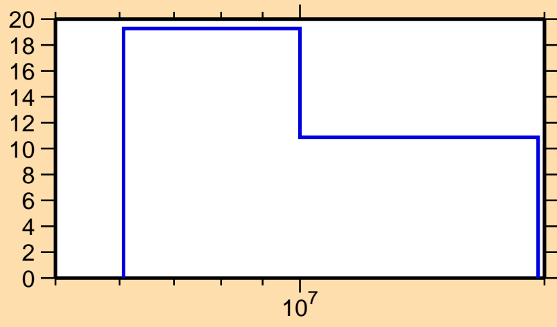
\Delta\sigma/\sigma vs. E for ^{123}\text{Te}(n,2n)
