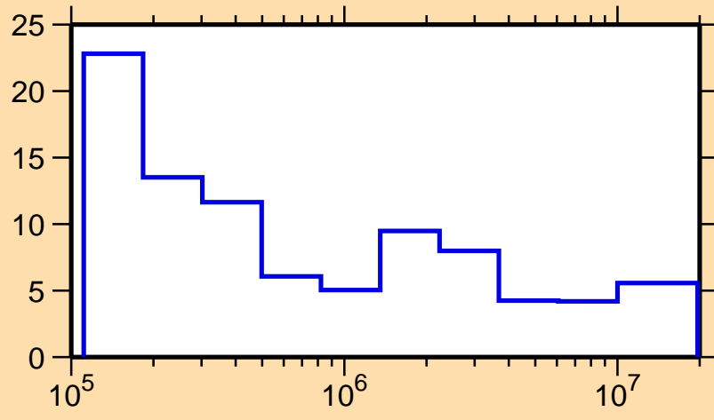
\Delta\sigma/\sigma vs. E for ^{123}\text{Te}(n,\text{tot.})
