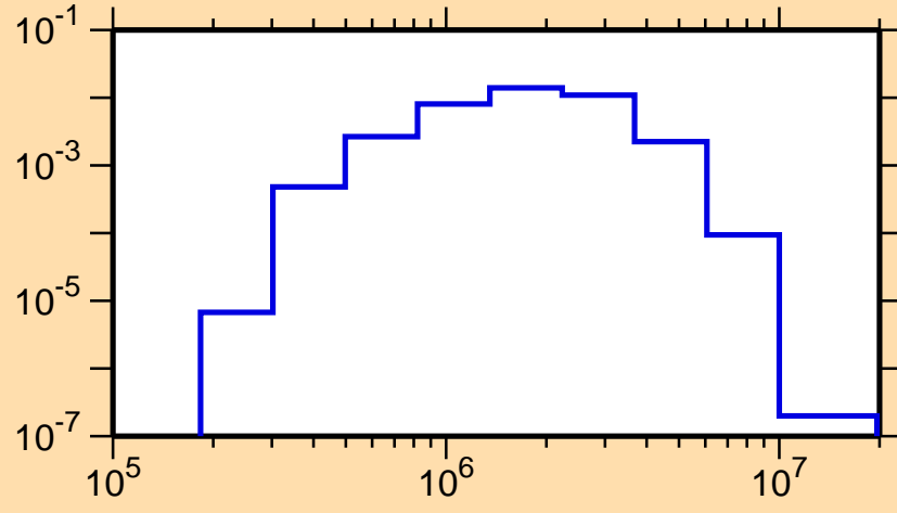
\sigma vs. E for ^{123}\text{Te}(n,n_2)
