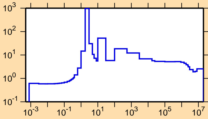
\sigma vs. E for ^{123}\text{Te}(n,\text{el.})
