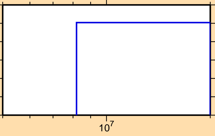
\sigma vs. E for ^{123}\text{Te}(n,\text{nd})
