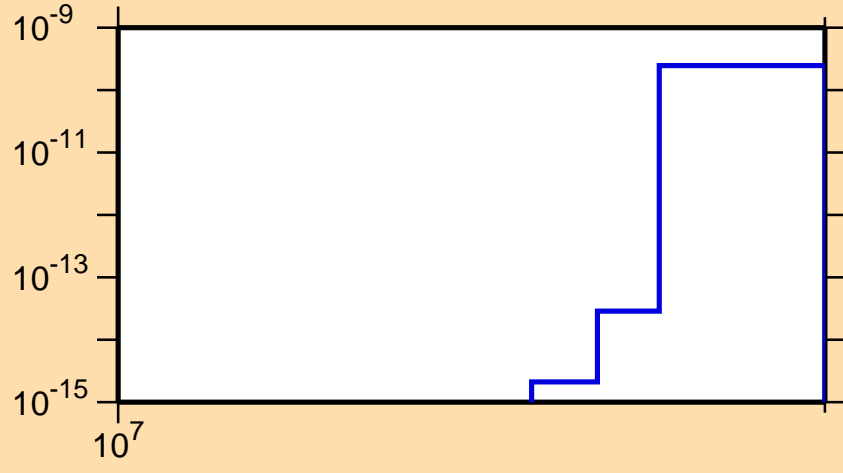
\sigma vs. E for ^{123}\text{Te}(n,nt)
