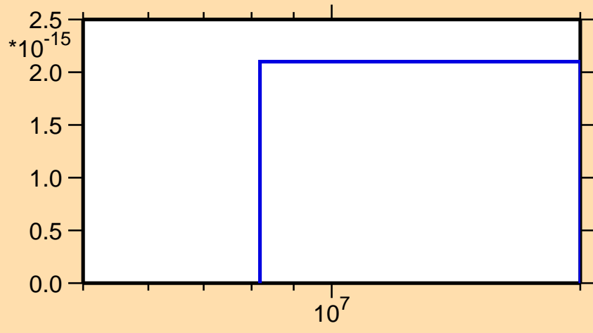
\sigma vs. E for ^{123}\text{Te}(n,pd)
