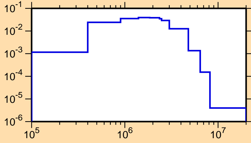
\sigma vs. E for ^{125}\text{Te}(n,n_3)
