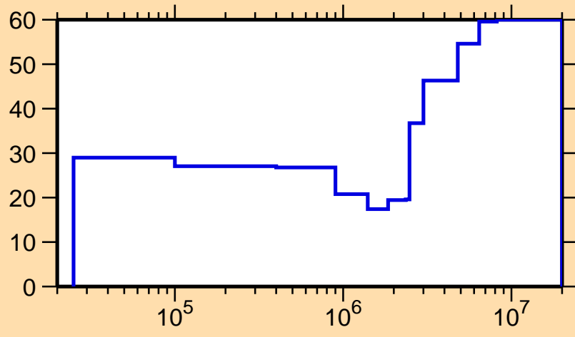
\Delta\sigma/\sigma vs. E for ^{125}\text{Te}(n,n_1)
