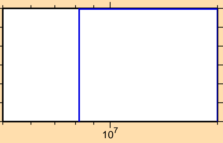
\sigma vs. E for ^{125}\text{Te}(n,d)
