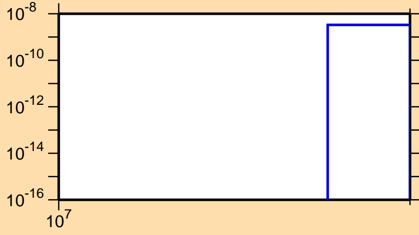
\sigma vs. E for ^{126}\text{Te}(n,\text{nd})
