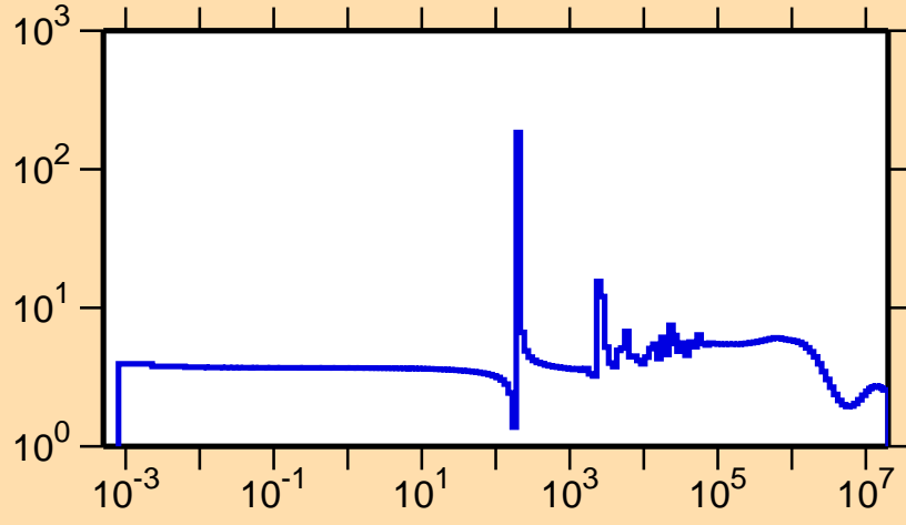
\sigma vs. E for ^{126}\text{Te}(n,\text{el.})
