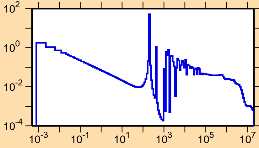
\sigma vs. E for ^{126}\text{Te}(n,\gamma)
