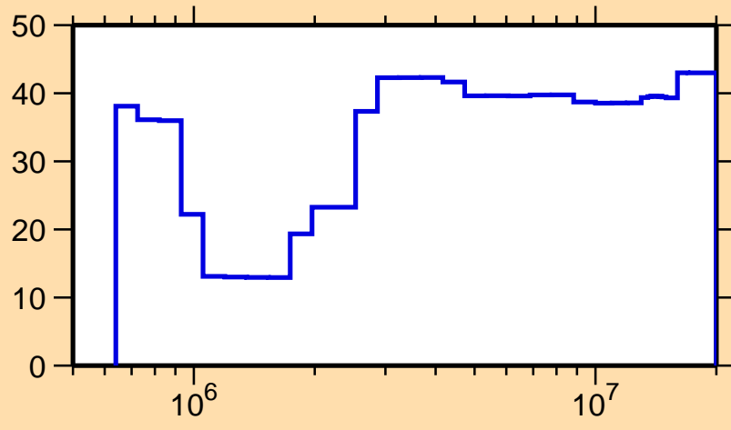
\Delta\sigma/\sigma vs. E for ^{126}\text{Te}(n,n_1)
