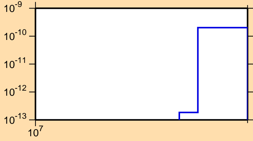
\sigma vs. E for ^{126}\text{Te}(n,2n\alpha)
