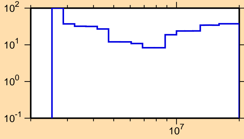
\Delta\sigma/\sigma vs. E for ^{126}\text{Te}(n,n\text{cont.})
