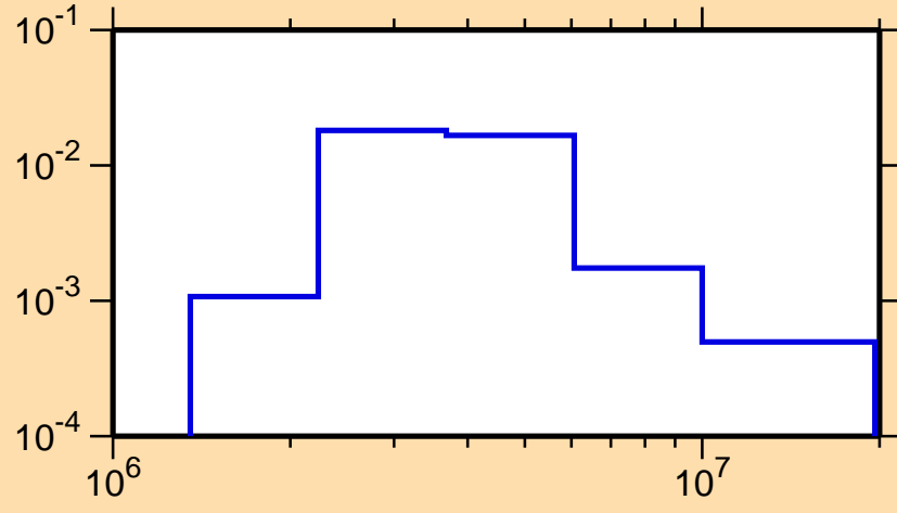
\sigma vs. E for ^{126}\text{Te}(n,n_4)
