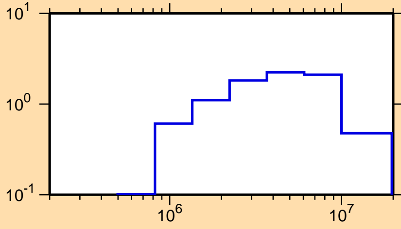
\sigma vs. E for ^{126}\text{Te}(n,\text{inel.})
