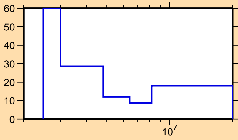
\Delta\sigma/\sigma vs. E for ^{126}\text{Te}(n,n\text{cont.})
