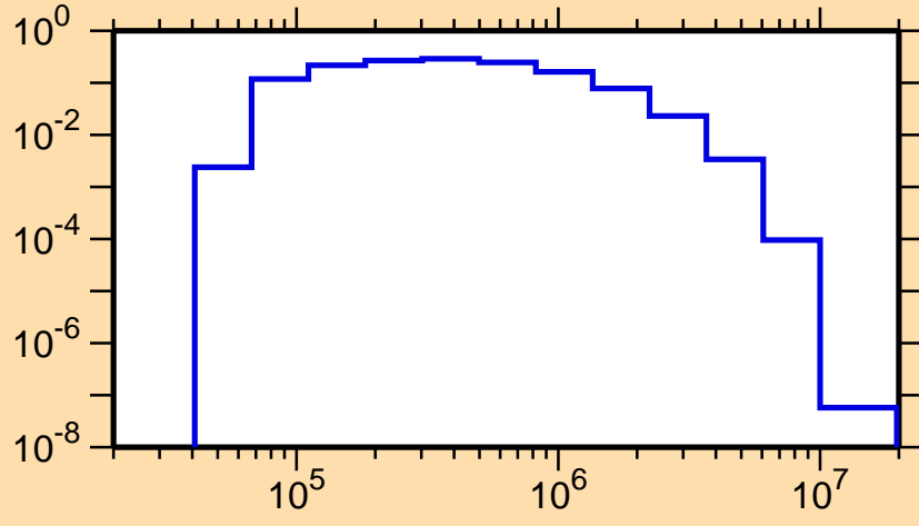
\sigma vs. E for ^{127}\text{Te}(n,n_1)
