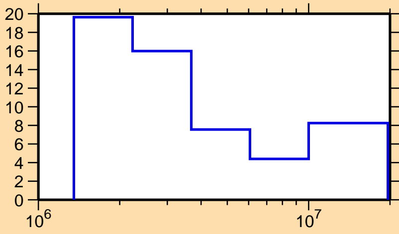
\Delta\sigma/\sigma vs. E for ^{127}\text{Te}(n,\text{tot.})
