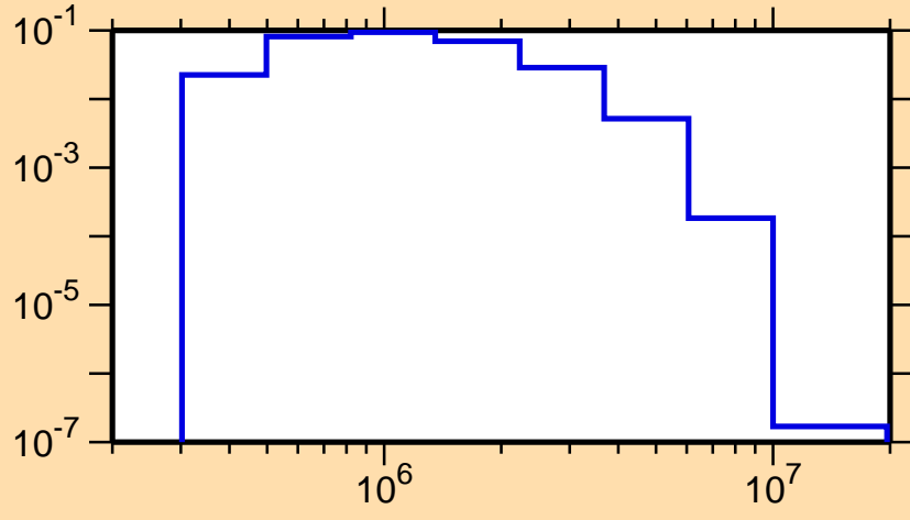
\sigma vs. E for ^{127}\text{Te}(n,n_3)
