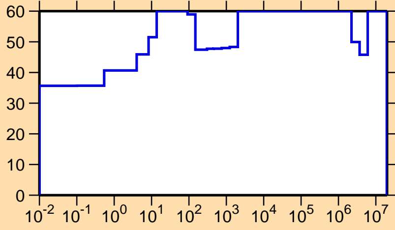
\Delta\sigma/\sigma vs. E for ^{127}\text{Te}(n,\gamma)
