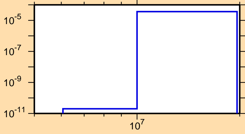
\sigma vs. E for ^{128}\text{Te}(n,\alpha)
