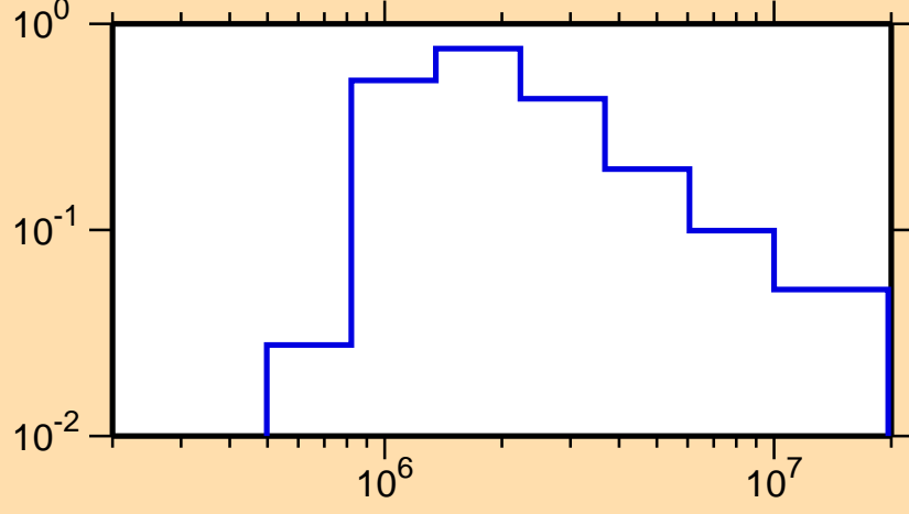
\sigma vs. E for ^{128}\text{Te}(n,n_1)
