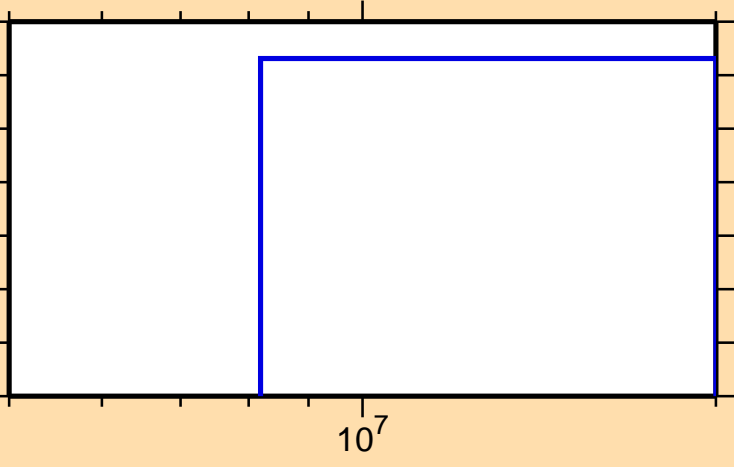
\sigma vs. E for ^{128}\text{Te}(n,np)
