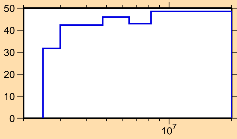
\Delta\sigma/\sigma vs. E for ^{128}\text{Te}(n, n_1)
