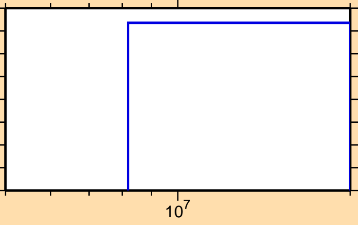
\sigma vs. E for ^{128}\text{Te}(n,\text{nd})
