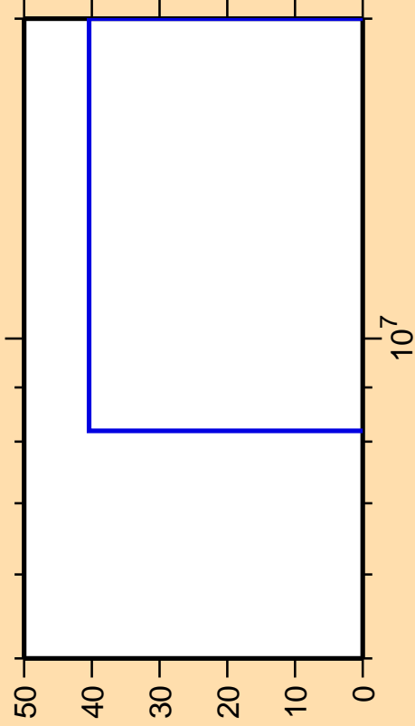
\Delta\sigma/\sigma vs. E for ^{128}\text{Te}(n,np)
