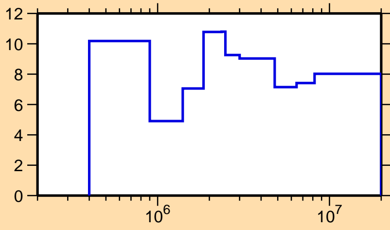
\Delta\sigma/\sigma vs. E for ^{128}\text{Te}(n,\text{el.})
