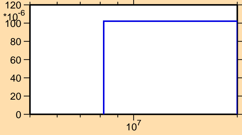
\sigma vs. E for ^{128}\text{Te}(n,d)
