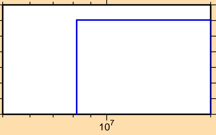
\sigma vs. E for ^{128}\text{Te}(n,2np)
