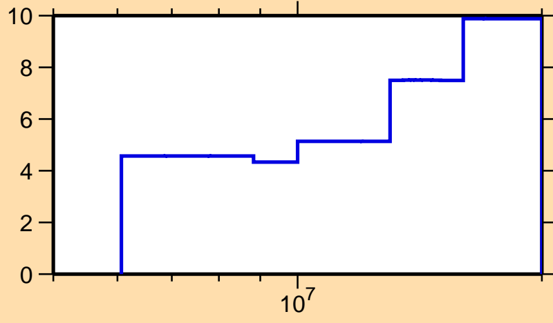
\Delta\sigma/\sigma vs. E for ^{129}\text{Te}(n,\text{tot.})
