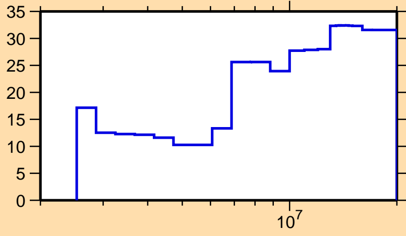
\Delta\sigma/\sigma vs. E for ^{129}\text{Te}(n,n\text{cont.})
