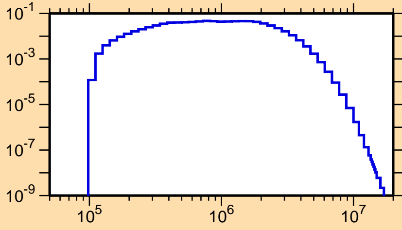
\sigma vs. E for ^{129}\text{Te}(n,n_1)
