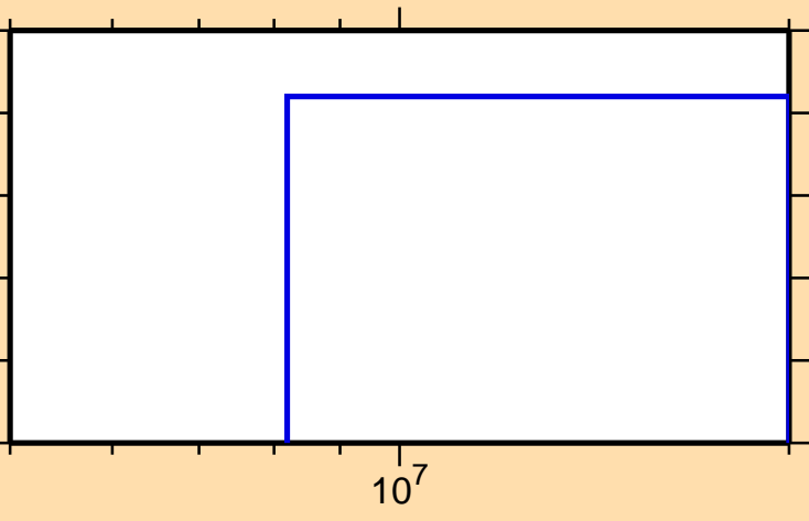
\sigma vs. E for ^{129}\text{Te}(n,np)
