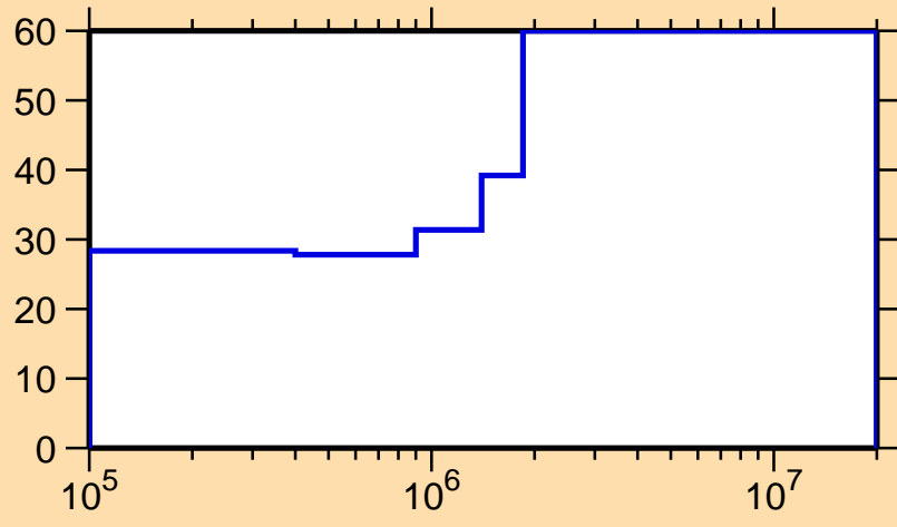
\Delta\sigma/\sigma vs. E for ^{129}\text{Te}(n,n_1)
