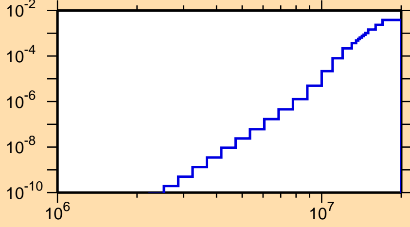
\sigma vs. E for ^{129}\text{Te}(n,\alpha)
