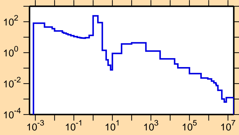
\sigma vs. E for ^{129}\text{Te}(n,\gamma)
