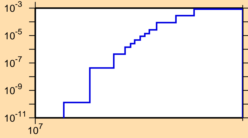
\sigma vs. E for ^{130}\text{Te}(n,np)
