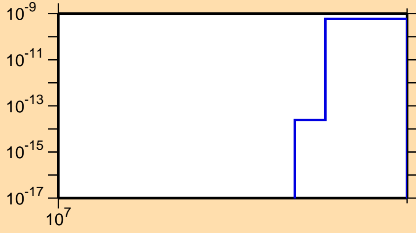
\sigma vs. E for ^{130}\text{Te}(n,\text{nd})
