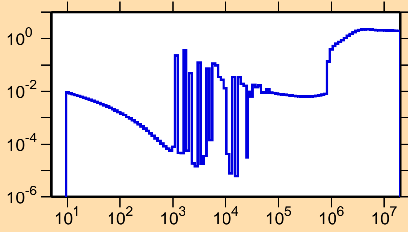
\sigma vs. E for ^{130}\text{Te}(n,\text{nonel.})
