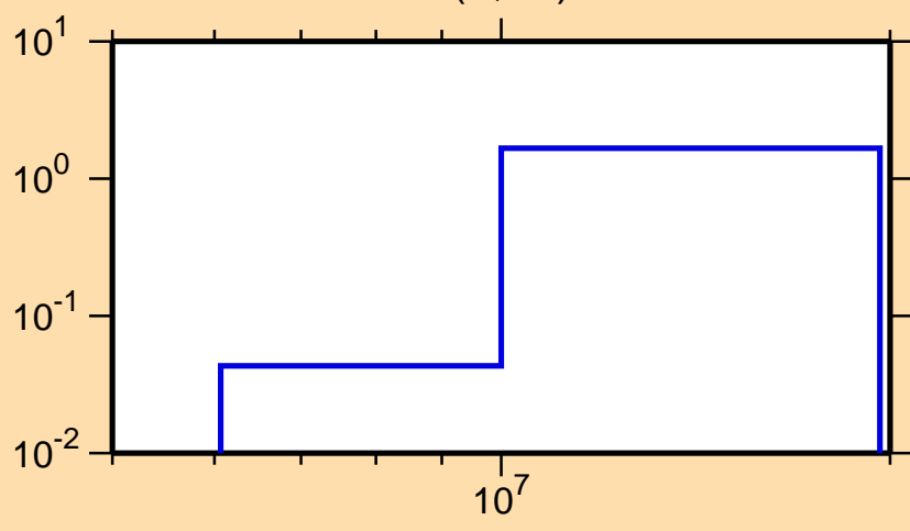
\sigma vs. E for ^{130}\text{Te}(n,2n)
