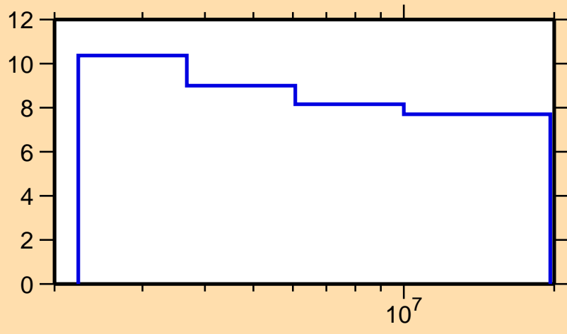
\Delta\sigma/\sigma vs. E for ^{130}\text{Te}(n,n\text{onel.})
