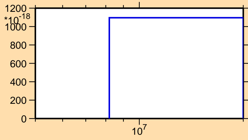
\sigma vs. E for ^{130}\text{Te}(n,\text{He3})
