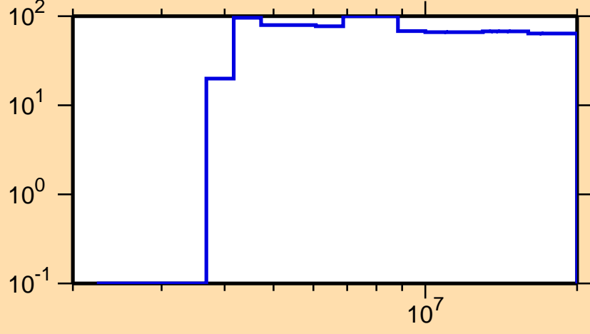
\Delta\sigma/\sigma vs. E for ^{131}\text{Te}(n,p)
