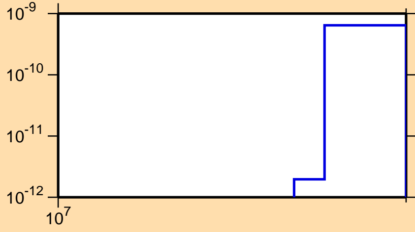
\sigma vs. E for ^{131}\text{Te}(n,2n\alpha)
