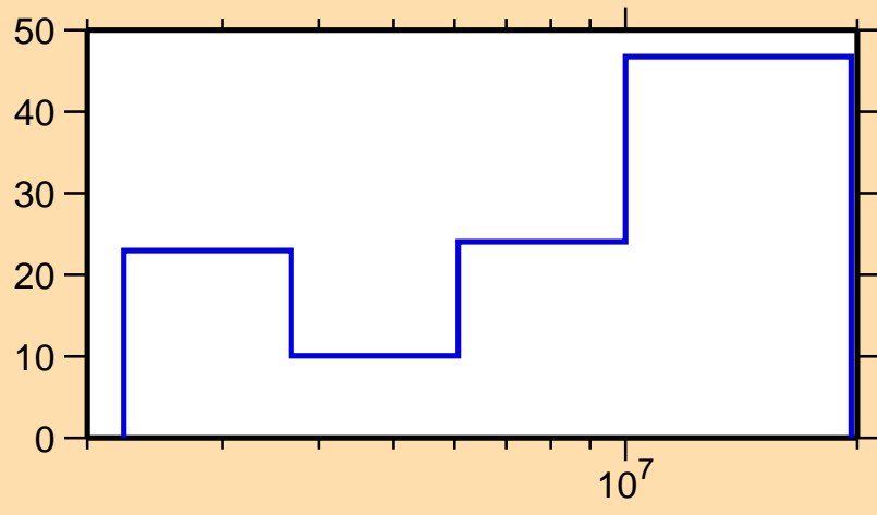
\Delta\sigma/\sigma vs. E for ^{131}\text{Te}(n,n\text{cont.})
