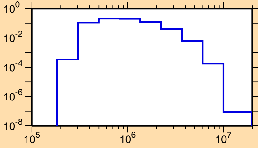
\sigma vs. E for ^{131}\text{Te}(n,n_2)
