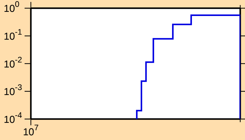
\sigma vs. E for ^{131}\text{Te}(n,3n)
