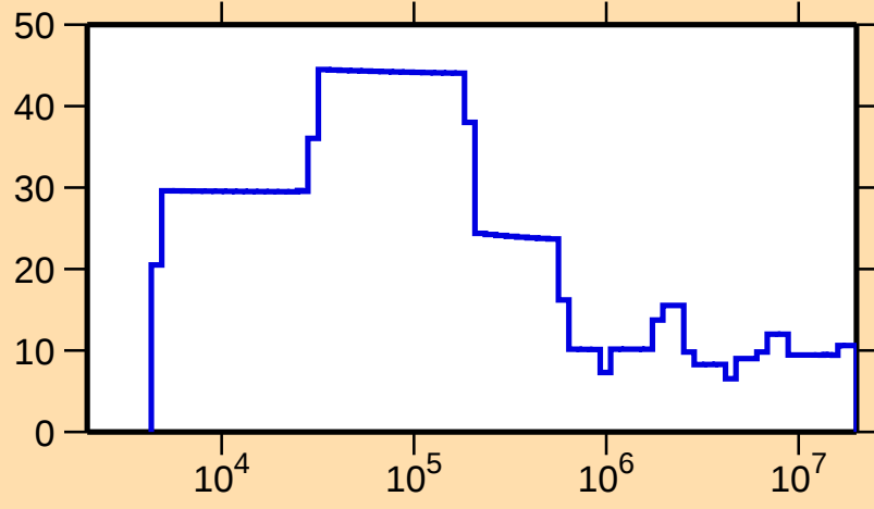
\Delta\sigma/\sigma vs. E for ^{131}\text{Te}(n,\text{el.})
