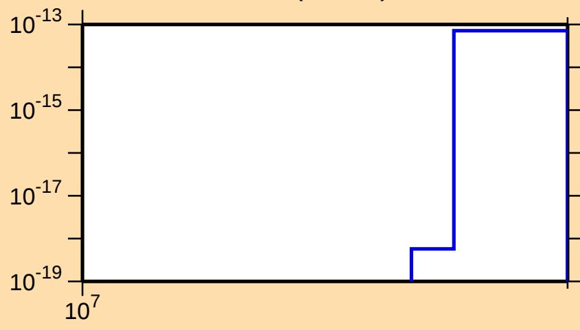
\sigma vs. E for ^{131}\text{Te}(n,\text{He3})
