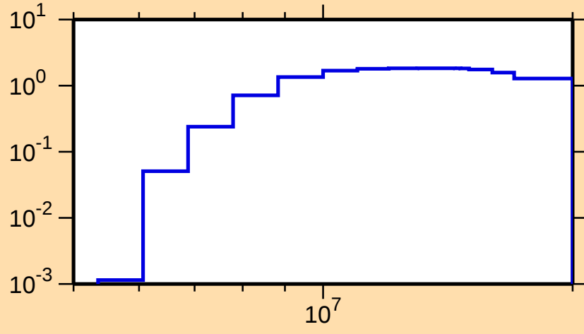
\sigma vs. E for ^{131}\text{Te}(n,2n)
