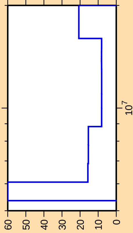
\Delta\sigma/\sigma vs. E for ^{131}\text{Te}(n,2n)
