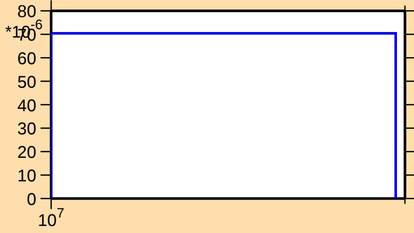
\sigma vs. E for ^{131}\text{Te}(n,np)
