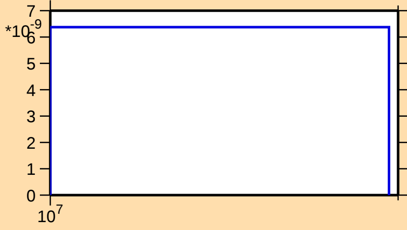
\sigma vs. E for ^{131}\text{Te}(n,\text{nd})
