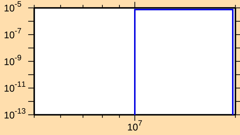
\sigma vs. E for ^{131}\text{Te}(n,n\alpha)
