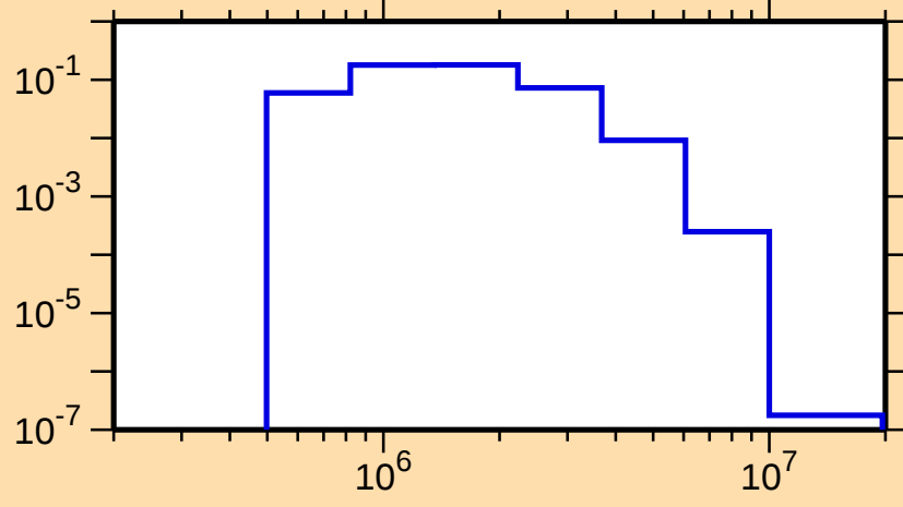
\sigma vs. E for ^{131}\text{Te}(n,n_4)
