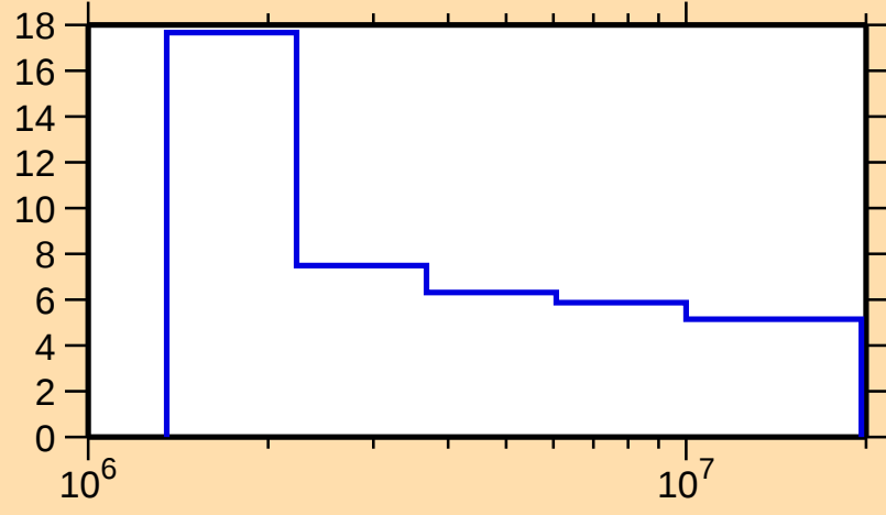
\Delta\sigma/\sigma vs. E for ^{131}\text{Te}(\text{n},\text{nonel.})
