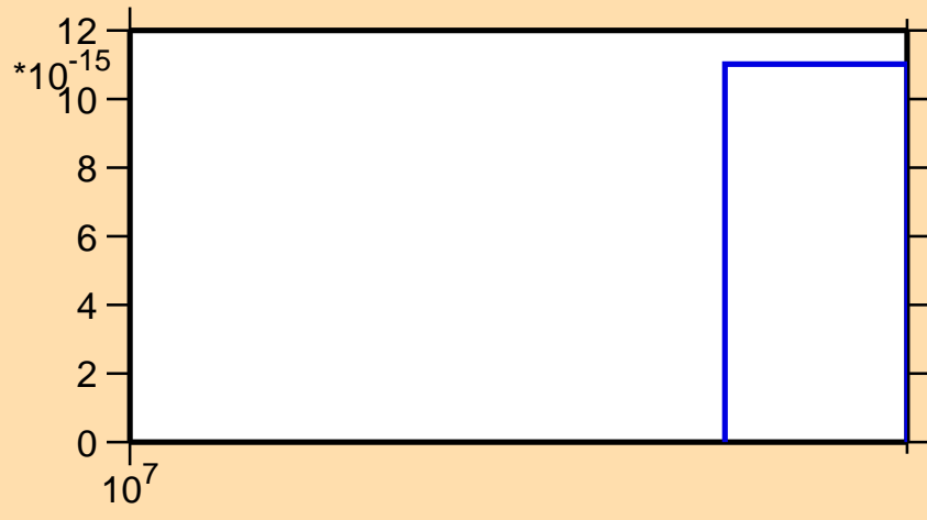
\sigma vs. E for ^{132}\text{Te}(n,2np)
