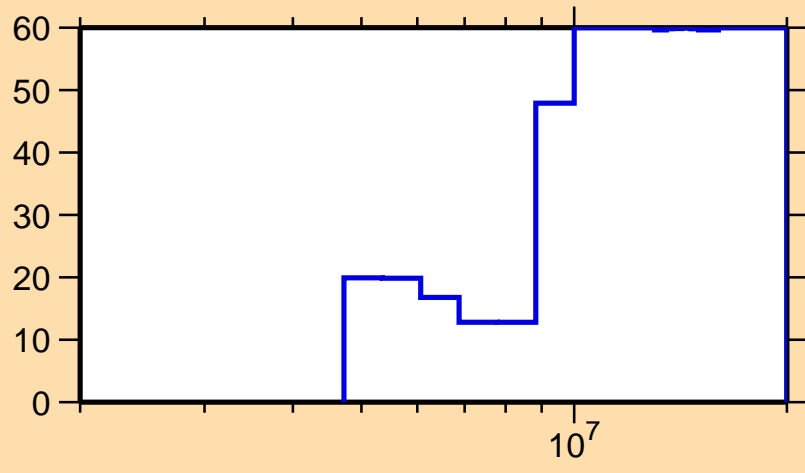
\Delta\sigma/\sigma vs. E for ^{132}\text{Te}(n,n\text{cont.})
