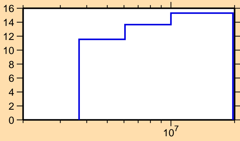
\Delta\sigma/\sigma vs. E for ^{132}\text{Te}(n,el.)
