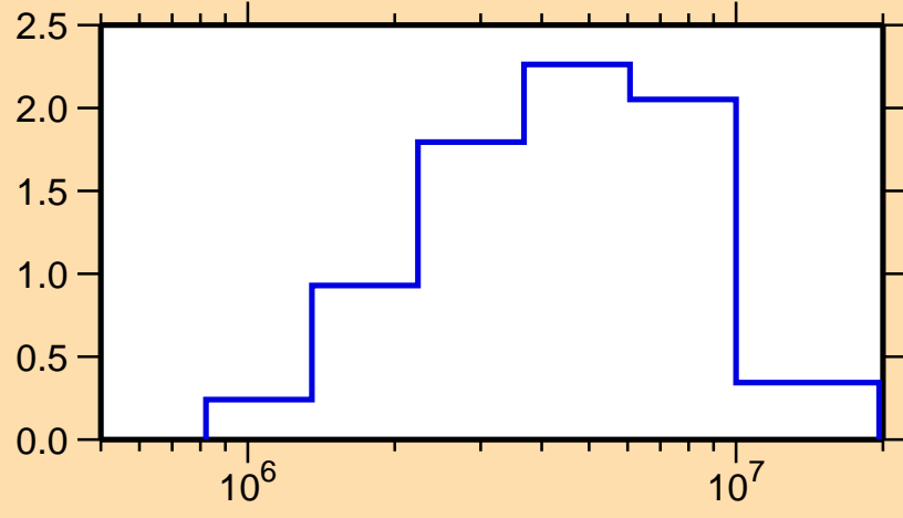
\sigma vs. E for ^{132}\text{Te}(n,\text{inel.})
