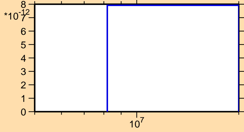
\sigma vs. E for ^{132}\text{Te}(n,nt)
