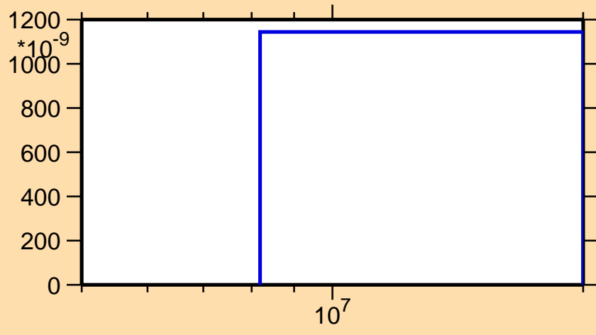
\sigma vs. E for ^{132}\text{Te}(n,n\alpha)
