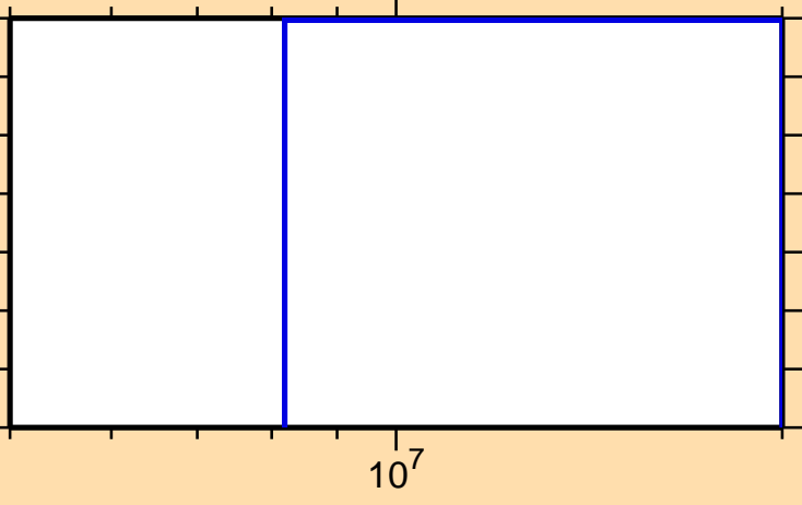
\sigma vs. E for ^{132}\text{Te}(n,d)
