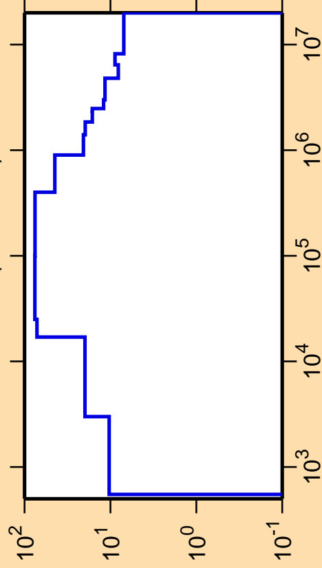
\Delta\sigma/\sigma vs. E for ^{132}\text{Te}(n,\text{nonel.})
