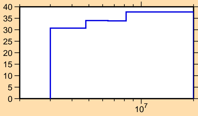
\Delta\sigma/\sigma vs. E for ^{132}\text{Te}(n,n_1)
