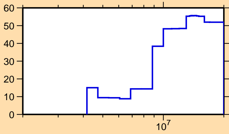
\Delta\sigma/\sigma vs. E for ^{133}\text{Te}(n,n\text{cont.})
