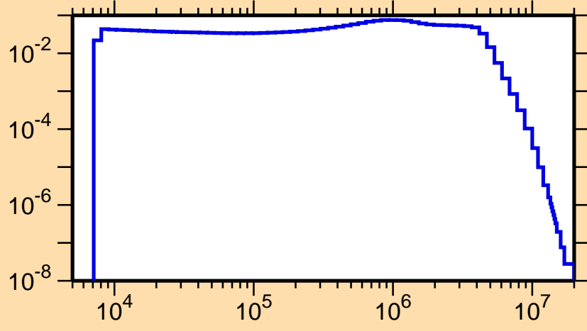
\sigma vs. E for ^{133}\text{Te}(n,n_1)
