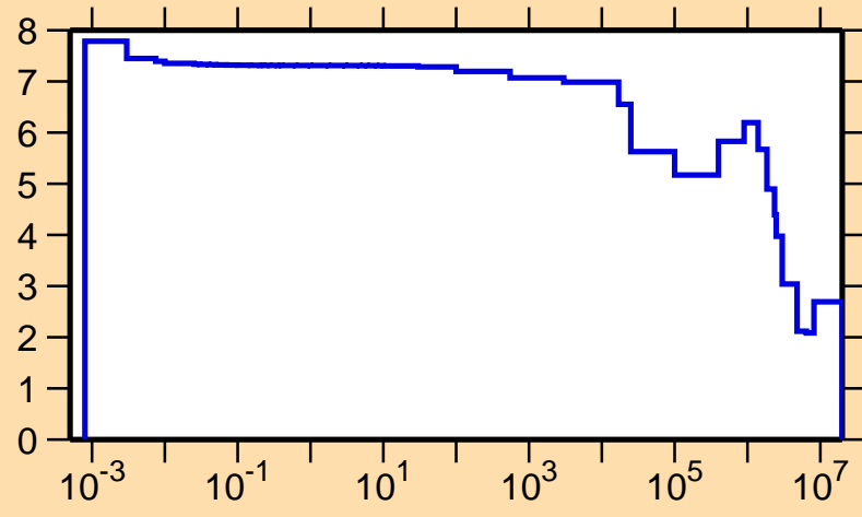
\sigma vs. E for ^{133}\text{Te}(n,\text{el.})
