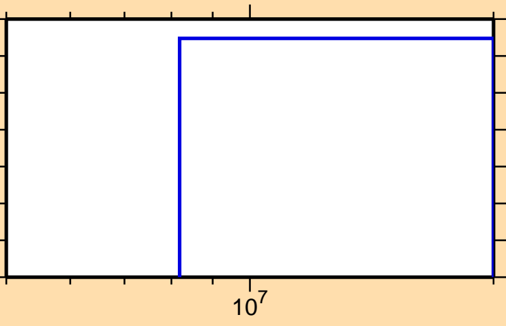
\sigma vs. E for ^{133}\text{Te}(n,np)
