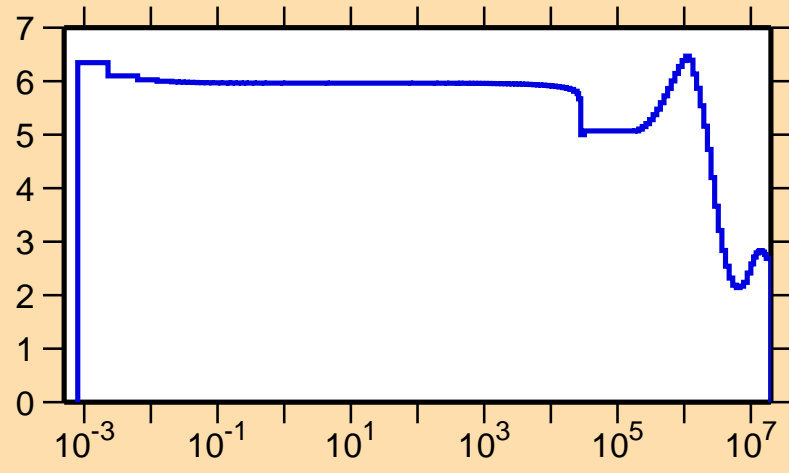
\sigma vs. E for ^{134}\text{Te}(n,\text{el.})
