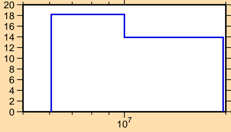
\Delta\sigma/\sigma vs. E for ^{134}\text{Te}(n,n\text{onel.})
