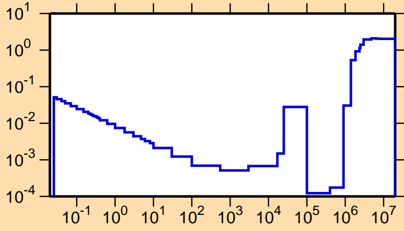
\sigma vs. E for ^{134}\text{Te}(n,\text{nonel.})
