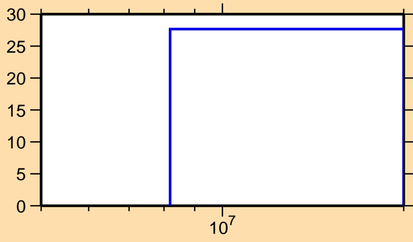
\Delta\sigma/\sigma vs. E for ^{134}\text{Te}(n,el.)
