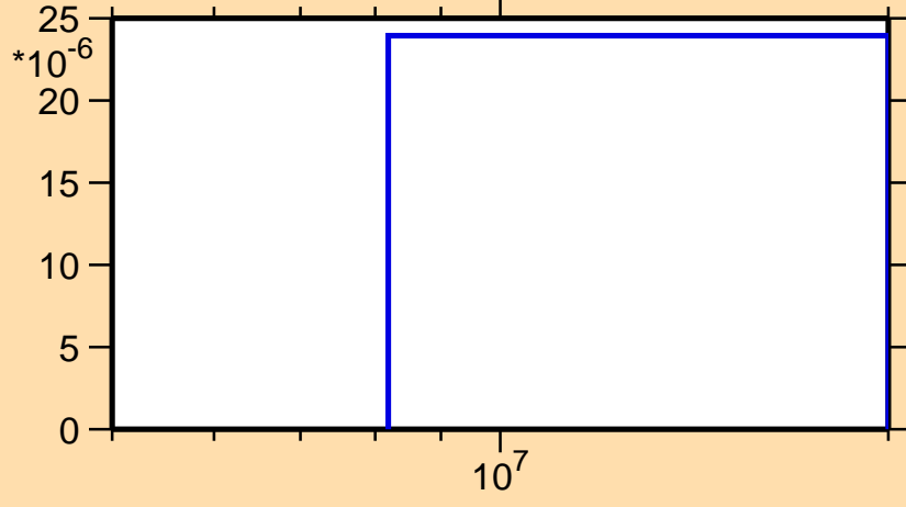
\sigma vs. E for ^{134}\text{Te}(n,d)
