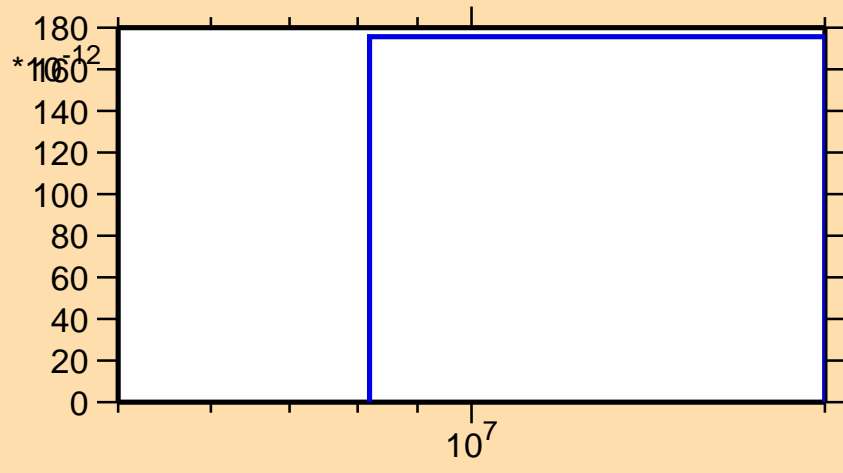
\sigma vs. E for ^{135}\text{Te}(n,2n\alpha)
