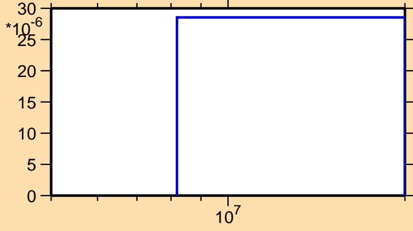
\sigma vs. E for ^{135}\text{Te}(n,n\alpha)
