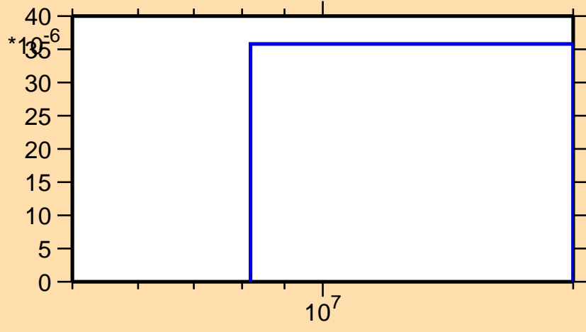
\sigma vs. E for ^{135}\text{Te}(n,d)
