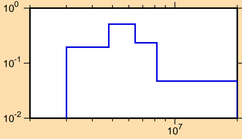
\sigma vs. E for ^{135}\text{Te}(n,n\text{cont.})
