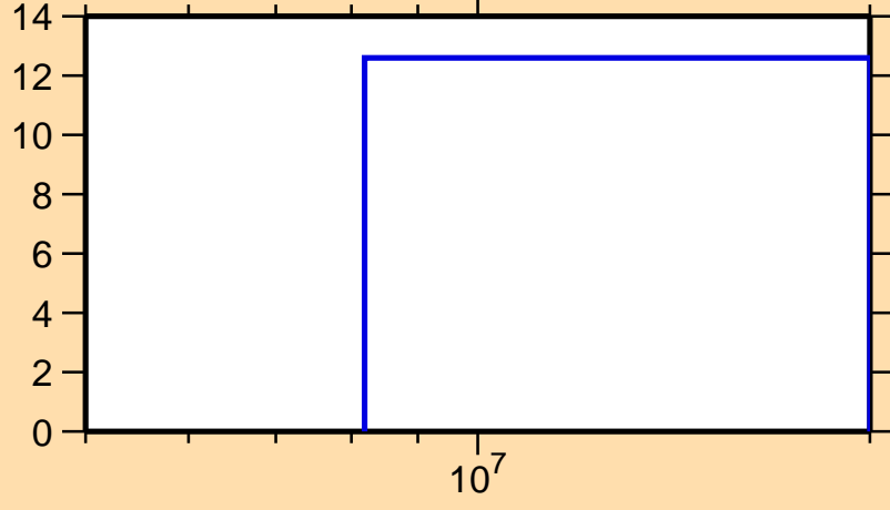
\Delta\sigma/\sigma vs. E for ^{135}\text{Te}(n,\text{tot.})
