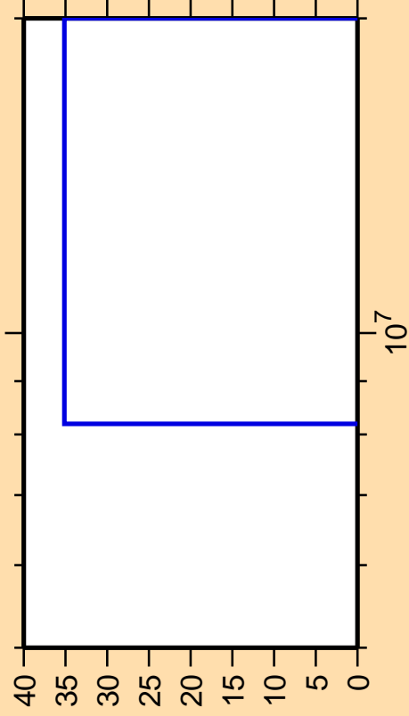
\Delta\sigma/\sigma vs. E for ^{135}\text{Te}(n,3n)
