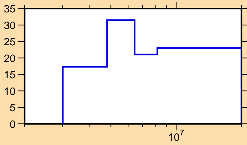
\Delta\sigma/\sigma vs. E for ^{135}\text{Te}(n,\text{el.})
