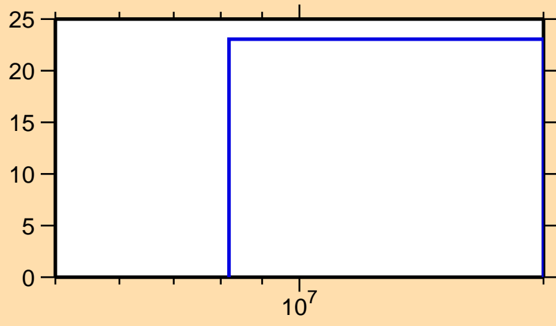
\Delta\sigma/\sigma vs. E for ^{135}\text{Te}(n,el.)
