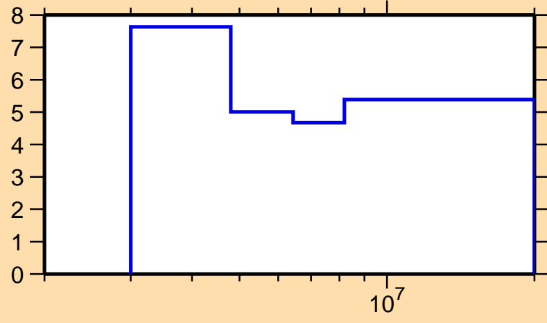
\Delta\sigma/\sigma vs. E for ^{135}\text{Te}(n,\text{nonel.})
