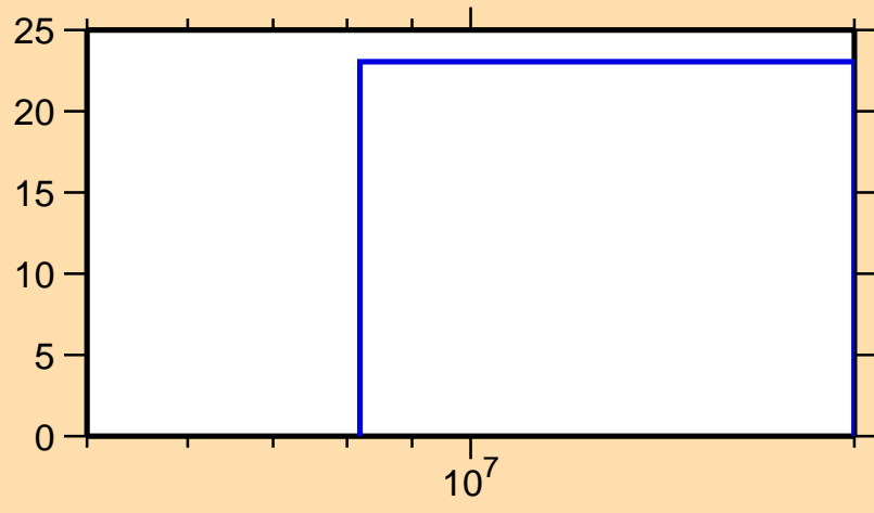
\Delta\sigma/\sigma vs. E for ^{135}\text{Te}(n,2n)
