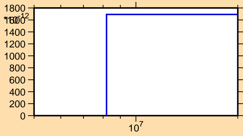
\sigma vs. E for ^{135}\text{Te}(n,2np)
