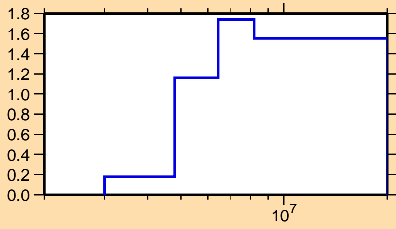
\sigma vs. E for ^{135}\text{Te}(n,2n)
