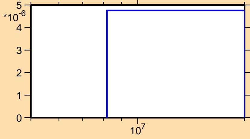
\sigma vs. E for ^{135}\text{Te}(n,np)
