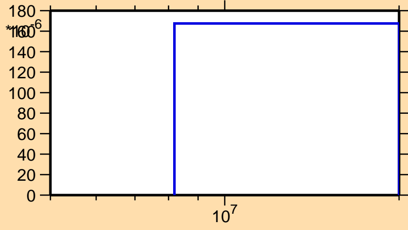
\sigma vs. E for ^{135}\text{Te}(n,p)
