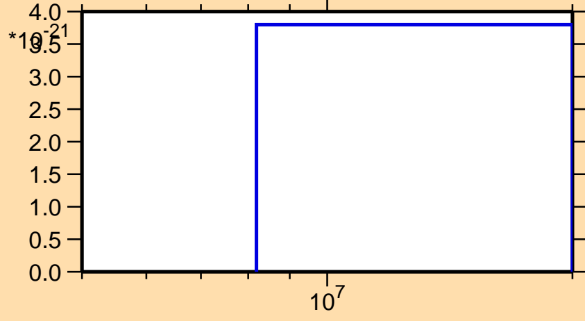
\sigma vs. E for ^{135}\text{Te}(\text{mt } 11)
