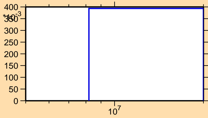
\sigma vs. E for ^{135}\text{Te}(n,3n)
