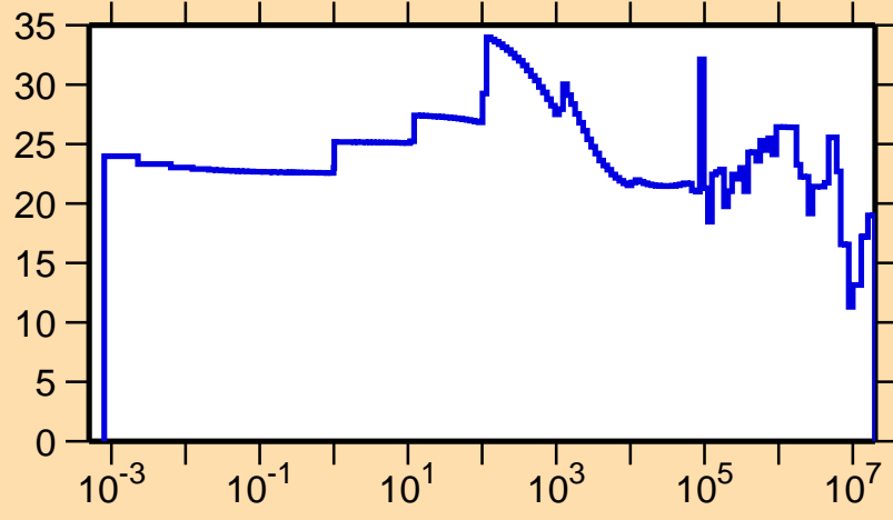
\Delta\sigma/\sigma vs. E for ^{136}\text{Te}(n,\text{tot.})
