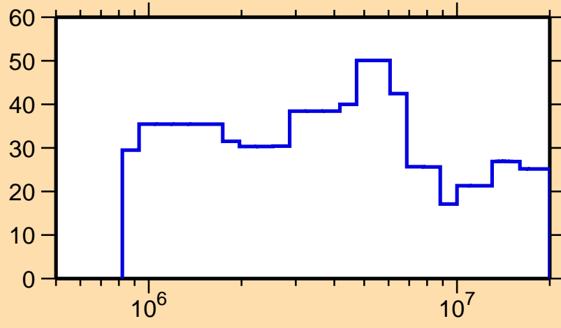
\Delta\sigma/\sigma vs. E for ^{136}\text{Te}(n,\text{el.})
