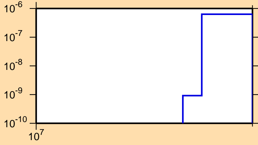
\sigma vs. E for ^{136}\text{Te}(n,\text{nd})
