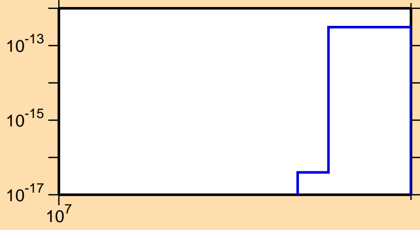
\sigma vs. E for ^{136}\text{Te} (mt 11)
