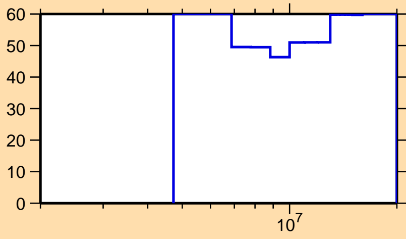
\Delta\sigma/\sigma vs. E for ^{136}\text{Te}(n,n\text{cont.})
