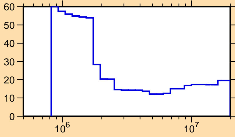
\Delta\sigma/\sigma vs. E for ^{136}\text{Te}(n,\text{nonel.})
