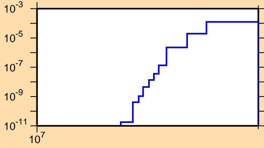
\sigma vs. E for ^{136}\text{Te}(n,nt)
