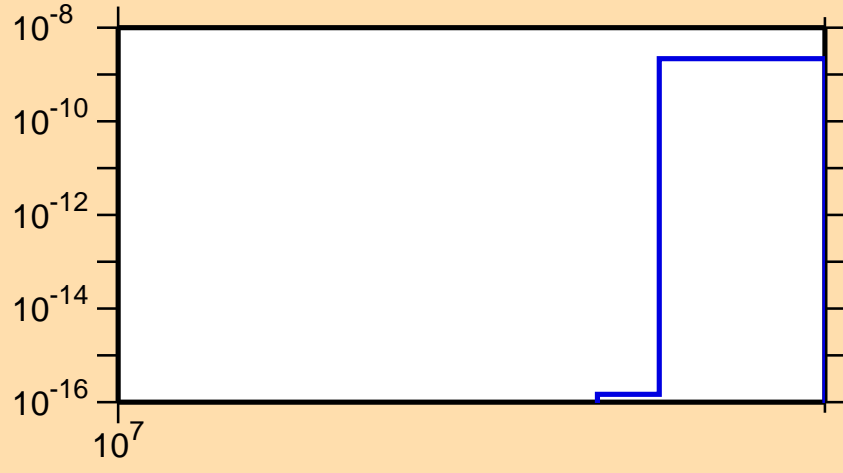
\sigma vs. E for ^{136}\text{Te}(n,2np)
