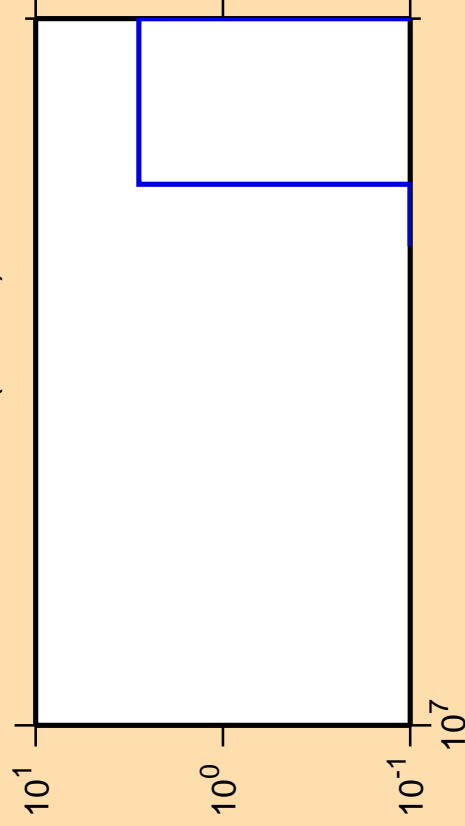
\Delta\sigma/\sigma vs. E for ^{136}\text{Te} (mt 11)
