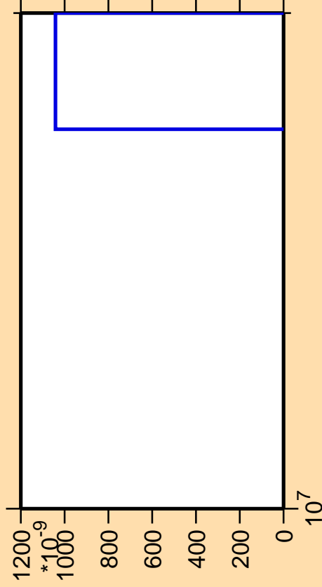
\Delta\sigma/\sigma vs. E for ^{136}\text{Te} (mt 42)
