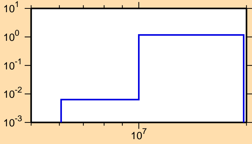
\sigma vs. E for ^{136}\text{Te}(n,3n)
