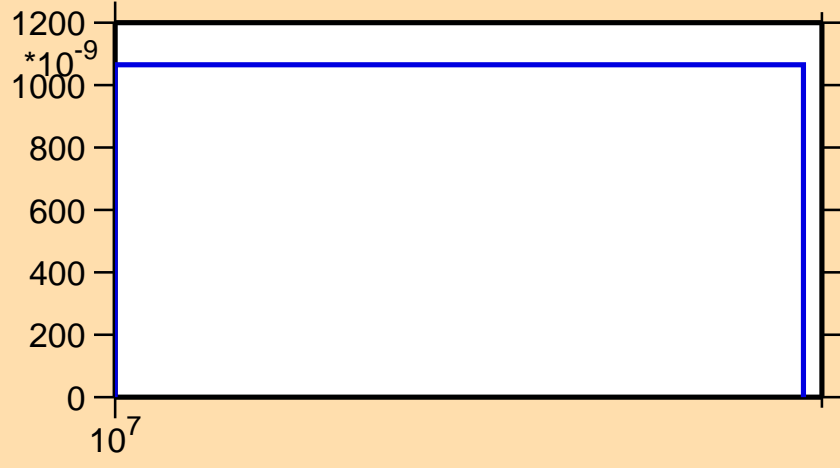
\sigma vs. E for ^{136}\text{Te}(n,np)
