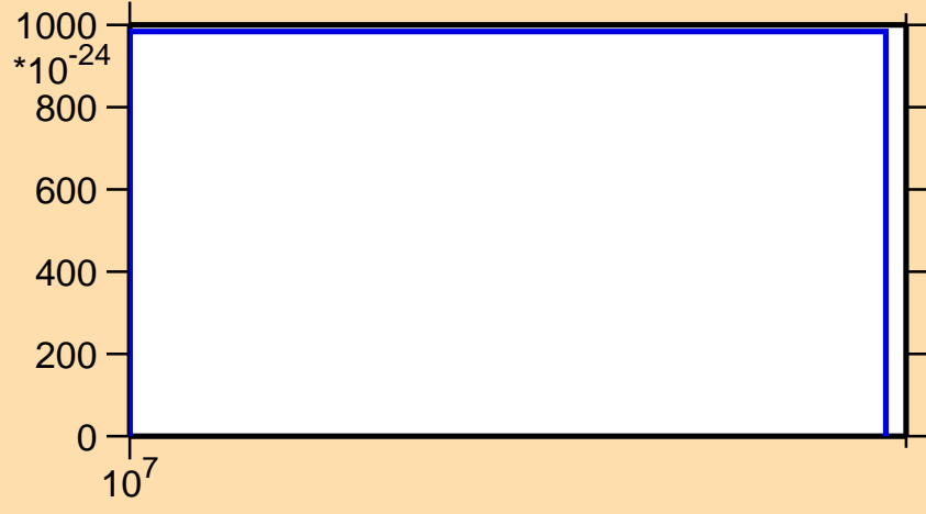
\sigma vs. E for ^{136}\text{Te} (mt 42)
