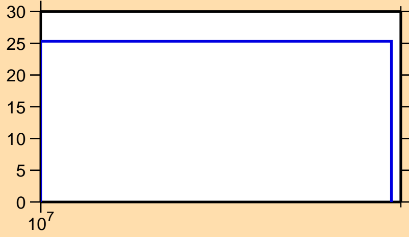
\Delta\sigma/\sigma vs. E for ^{136}\text{Te}(n,el.)
