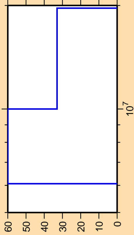
\Delta\sigma/\sigma vs. E for ^{136}\text{Te}(n,3n)
