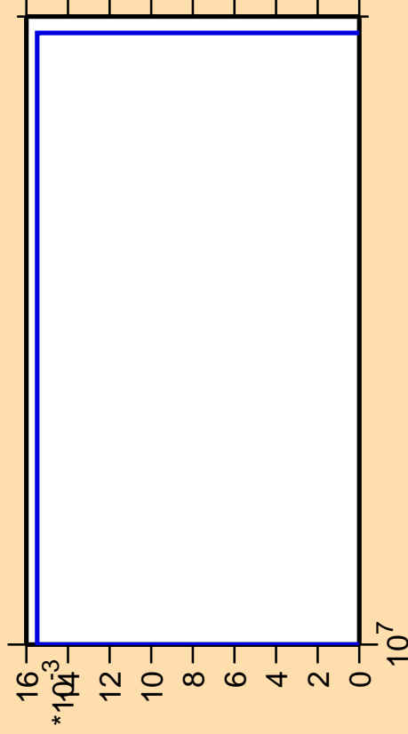
\Delta\sigma/\sigma vs. E for ^{136}\text{Te} (mt 11)
