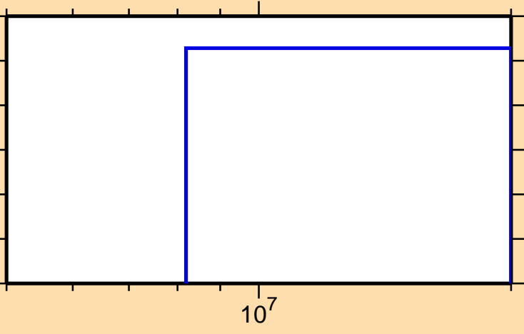
\sigma vs. E for ^{136}\text{Te}(n,t)
