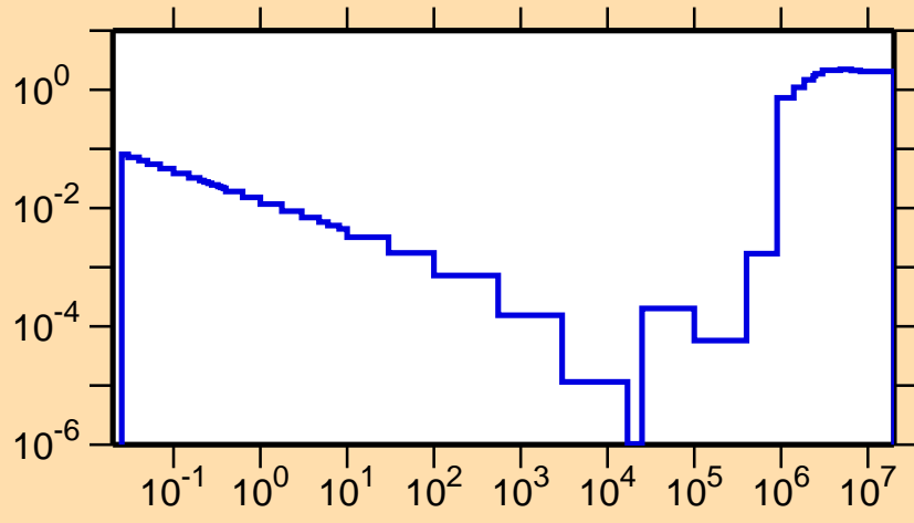
\sigma vs. E for ^{136}\text{Te}(n,\text{nonel.})
