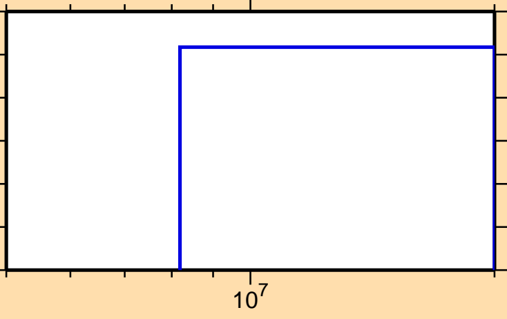
\sigma vs. E for ^{136}\text{Te}(n,\text{nd})
