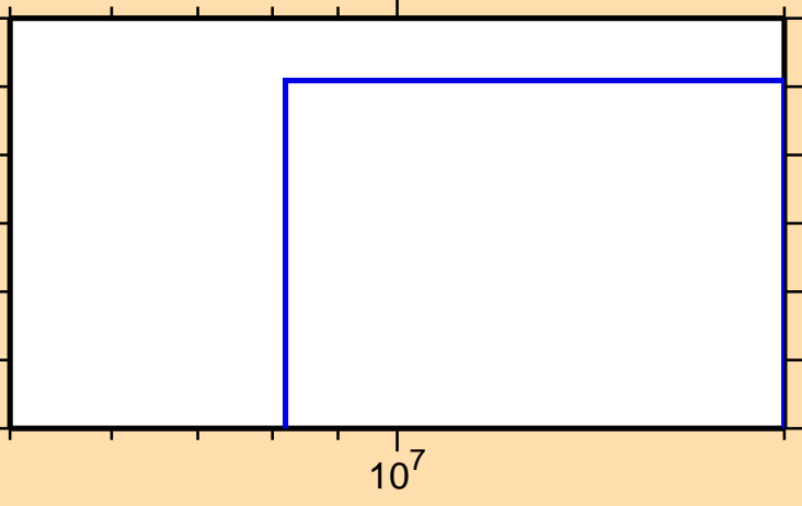
\sigma vs. E for ^{136}\text{Te}(\text{mt } 11)
