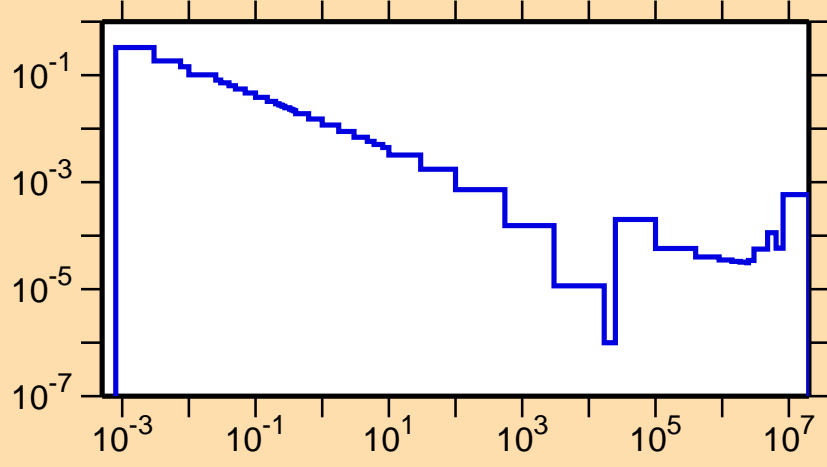
\sigma vs. E for ^{136}\text{Te}(n,\gamma)
