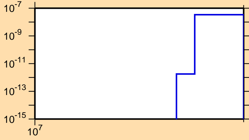
\sigma vs. E for ^{137}\text{Te}(n,2np)
