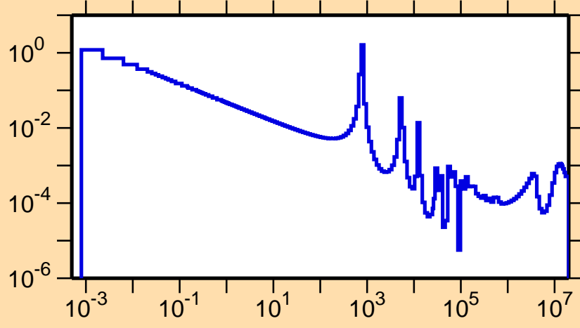
\sigma vs. E for ^{137}\text{Te}(n,\gamma)
