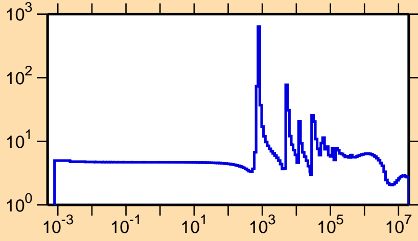
\sigma vs. E for ^{137}\text{Te}(n,\text{el.})
