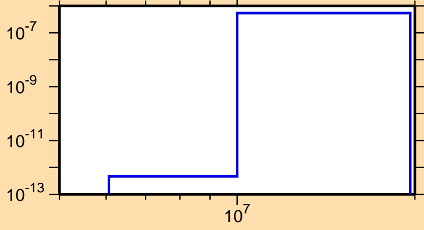
\sigma vs. E for ^{137}\text{Te}(n,2n\alpha)
