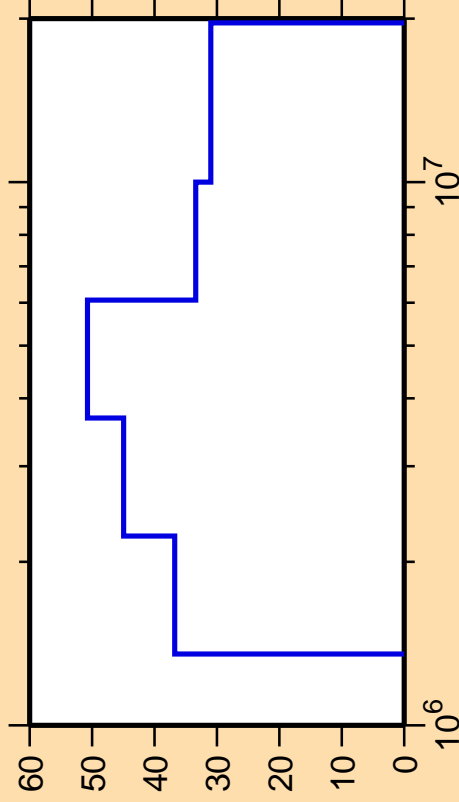
\Delta\sigma/\sigma vs. E for ^{137}\text{Te}(n,n_4)
