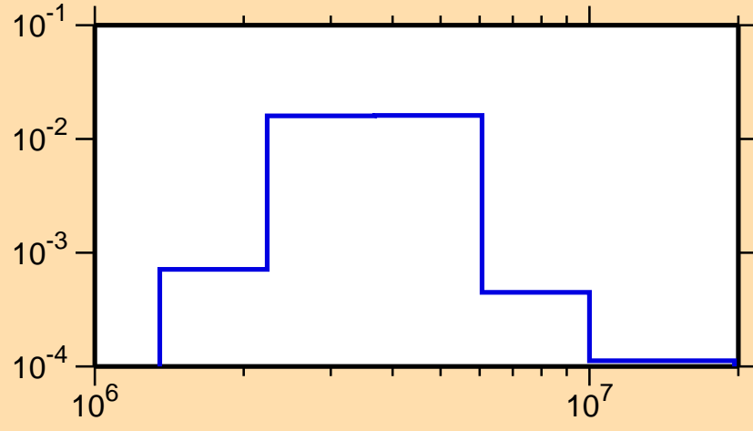
\sigma vs. E for ^{137}\text{Te}(n,n_4)
