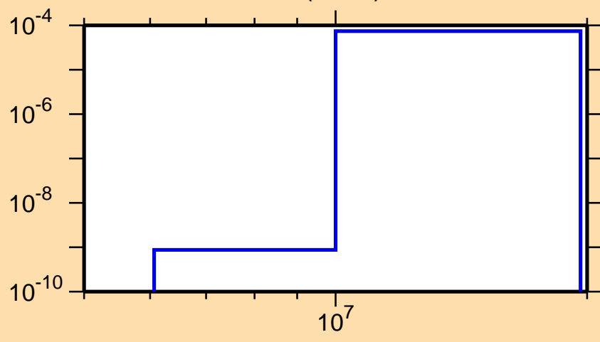
\sigma vs. E for ^{137}\text{Te}(n,n\alpha)
