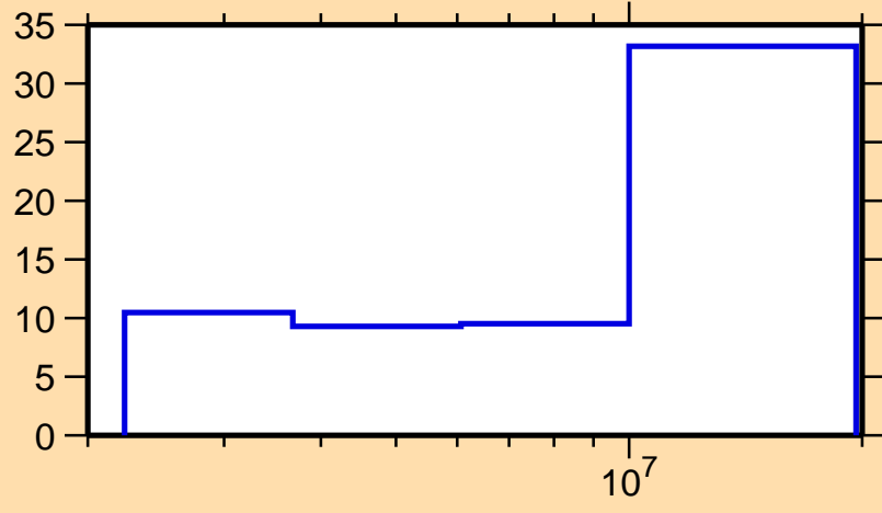
\Delta\sigma/\sigma vs. E for ^{137}\text{Te}(n,2n)
