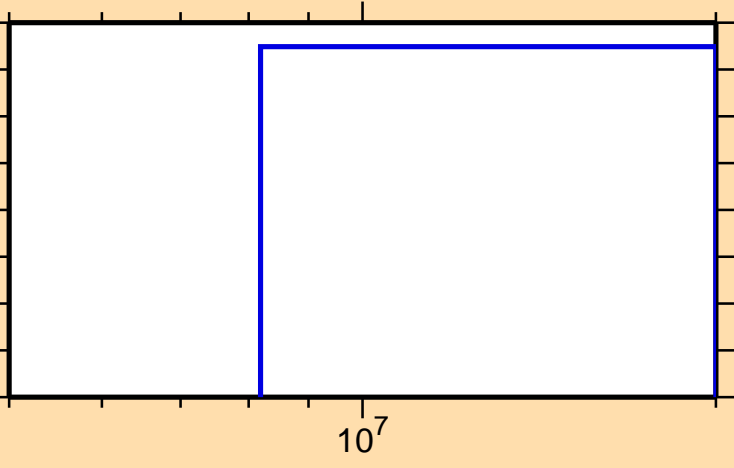
\sigma vs. E for ^{137}\text{Te}(n,t)
