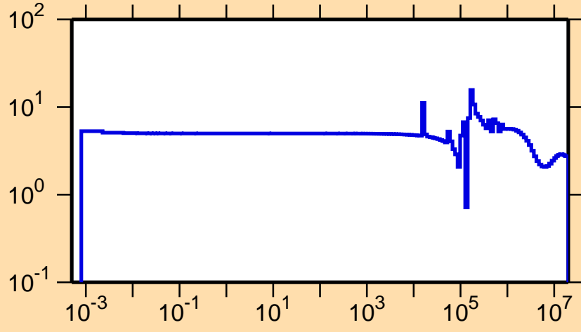
\sigma vs. E for ^{138}\text{Te}(n,\text{el.})
