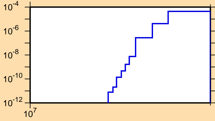
\sigma vs. E for ^{138}\text{Te}(n,nt)
