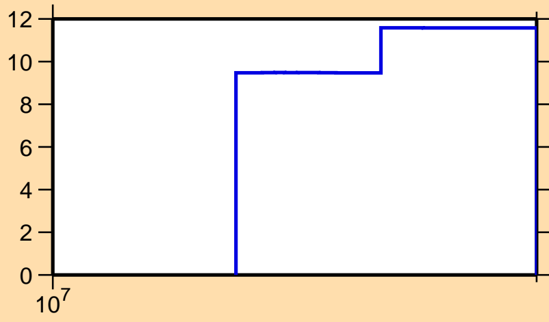
\Delta\sigma/\sigma vs. E for ^{138}\text{Te}(n,\text{tot.})
