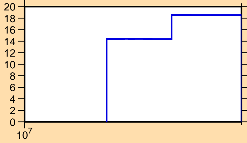
\Delta\sigma/\sigma vs. E for ^{138}\text{Te}(n,el.)
