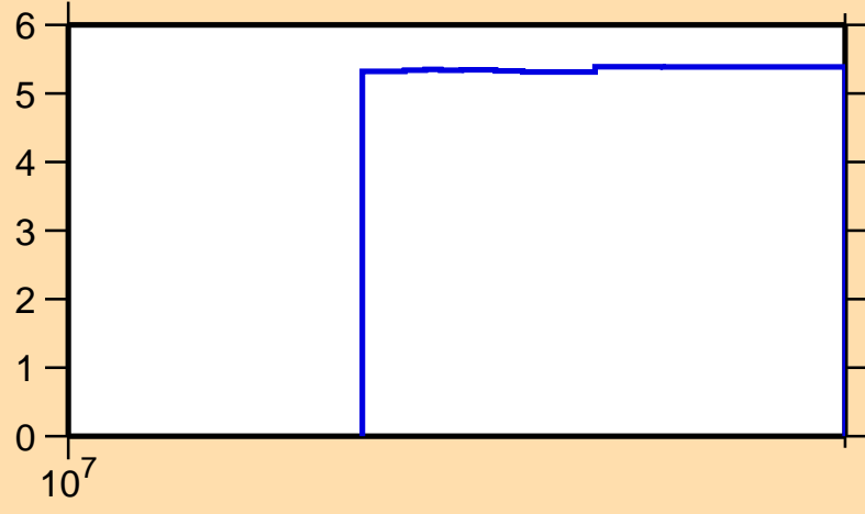
\Delta\sigma/\sigma vs. E for ^{138}\text{Te}(n,\text{nonel.})
