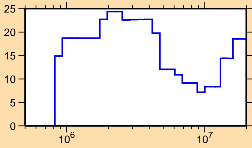
\Delta\sigma/\sigma vs. E for ^{138}\text{Te}(n,\text{el.})
