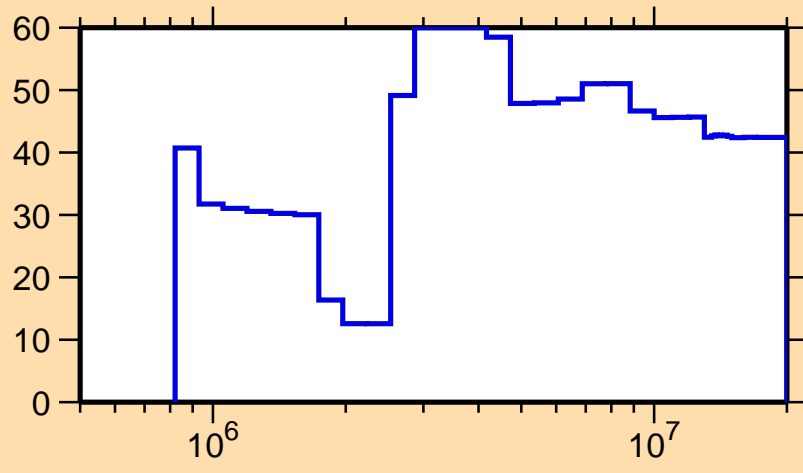
\Delta\sigma/\sigma vs. E for ^{138}\text{Te}(n,n_1)
