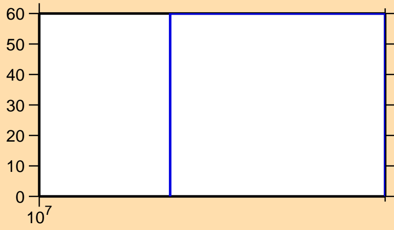
\Delta\sigma/\sigma vs. E for ^{138}\text{Te}(n,n\text{cont.})
