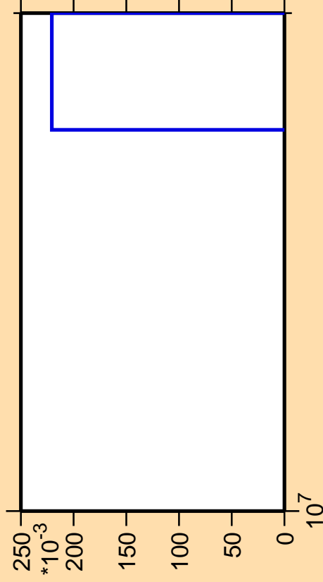
\Delta\sigma/\sigma vs. E for ^{138}\text{Te} (mt 11)
