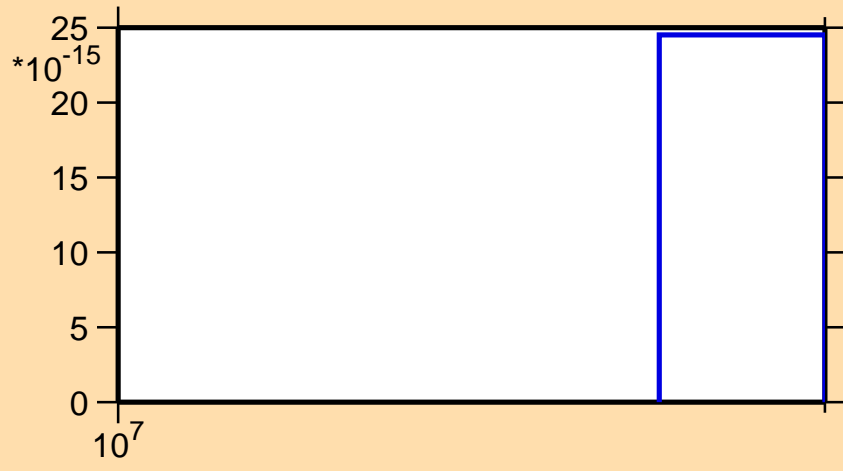
\sigma vs. E for ^{138}\text{Te} (mt 11)
