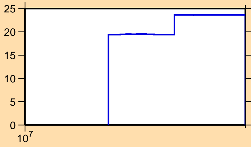
\Delta\sigma/\sigma vs. E for ^{138}\text{Te}(n,2n)
