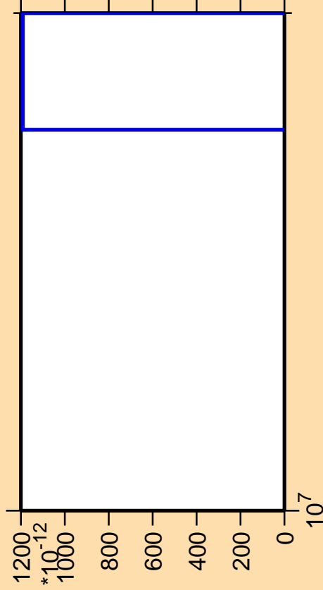
\Delta\sigma/\sigma vs. E for ^{138}\text{Te} (mt 42)
