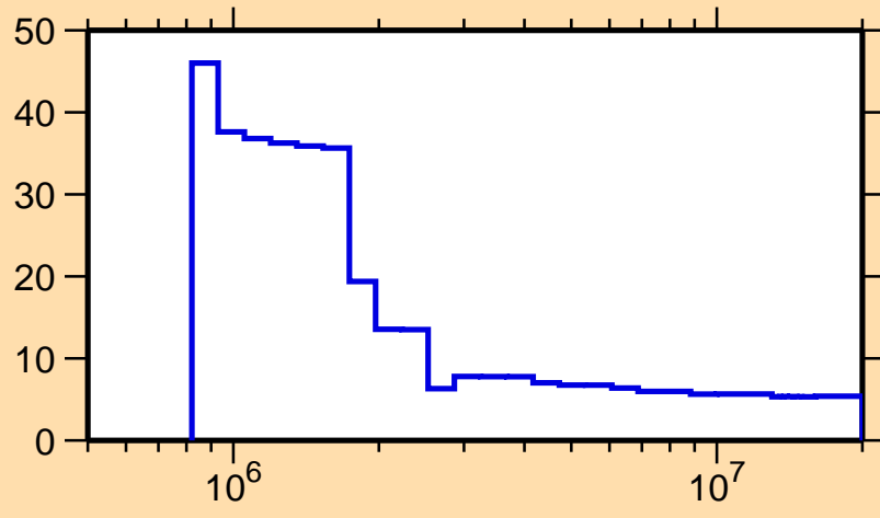
\Delta\sigma/\sigma vs. E for ^{138}\text{Te}(n,\text{nonel.})
