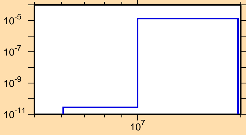
\sigma vs. E for ^{138}\text{Te}(n,n\alpha)
