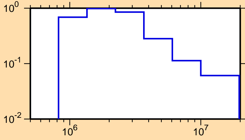
\sigma vs. E for ^{138}\text{Te}(n,n_1)
