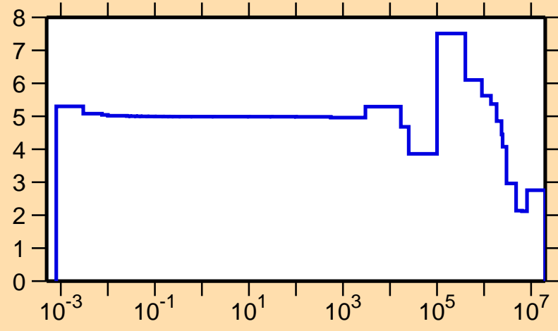
\sigma vs. E for ^{138}\text{Te}(n,\text{el.})
