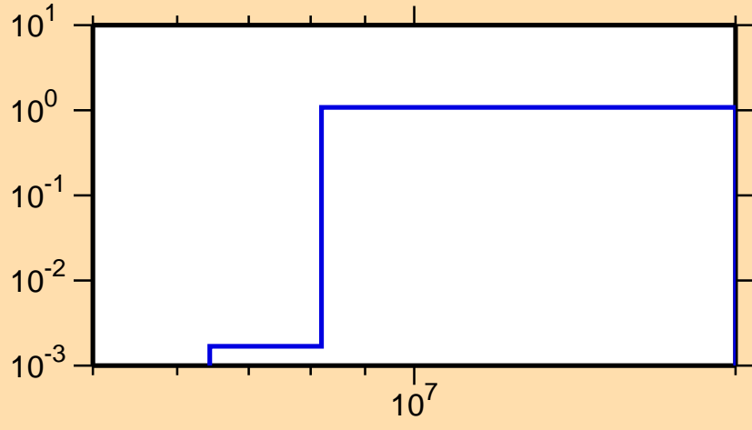
\sigma vs. E for ^{138}\text{Te}(n,3n)
