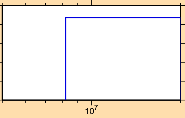
\sigma vs. E for ^{138}\text{Te}(n,np)
