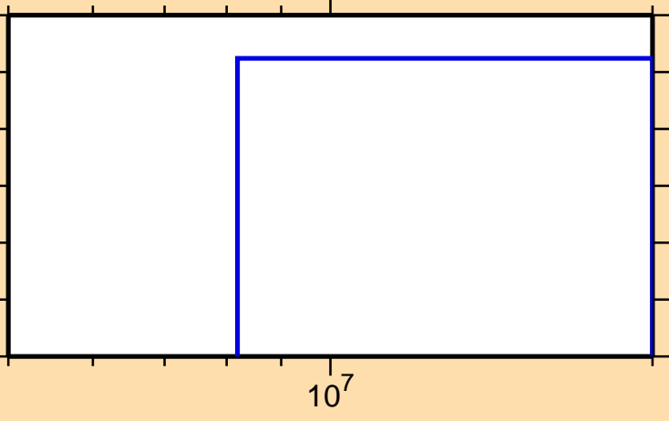
\sigma vs. E for ^{138}\text{Te}(n,2n\alpha)
