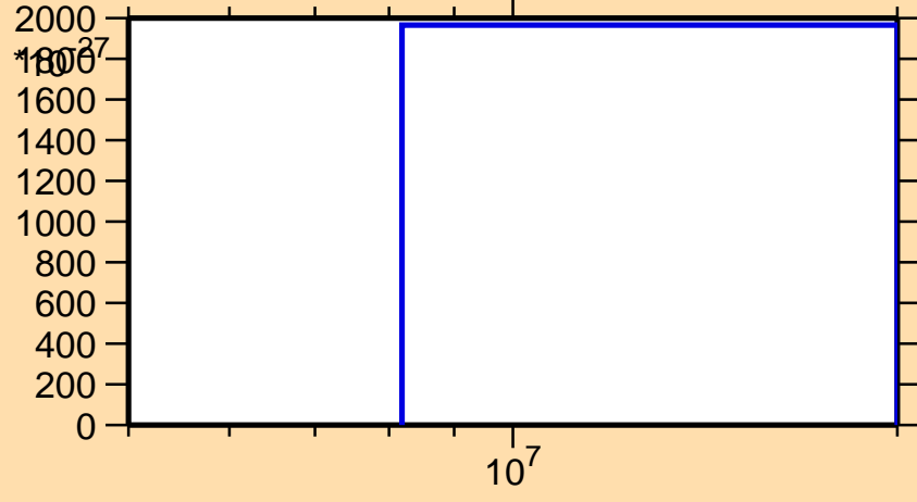
\sigma vs. E for ^{138}\text{Te} (mt 42)
