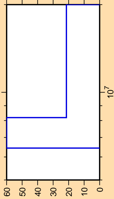
\Delta\sigma/\sigma vs. E for ^{138}\text{Te}(n,3n)
