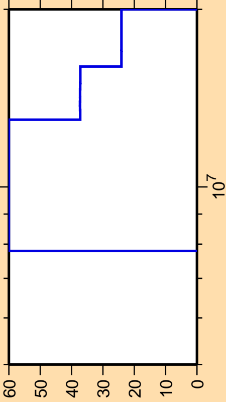
\Delta\sigma/\sigma vs. E for ^{215}\text{Th}(n,2n)
