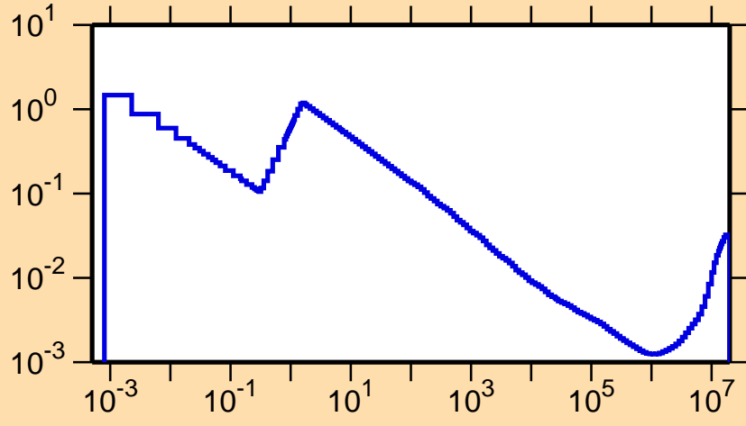
\sigma vs. E for ^{215}\text{Th}(n,\alpha)
